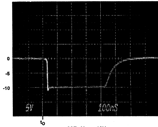
FIGURE 22. V_O - OUTPUT SWITCHING WAVEFORMS
