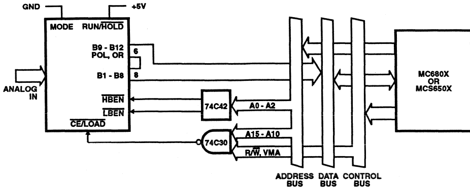
FIGURE 18. DIRECT ICL7109 - MC680X BUS INTERFACE
