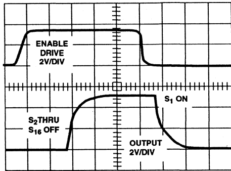
FIGURE 10C. ENABLE DELAY t_{ON(EN)} , t_{OFF(EN)}
