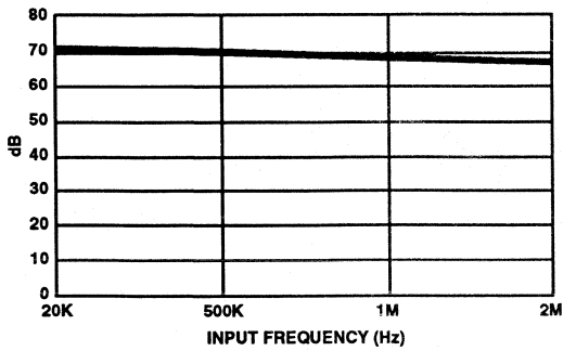
FIGURE 4. TYPICAL SNR vs INPUT FREQUENCY
