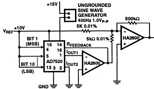
FIGURE 3. POWER SUPPLY REJECTION
