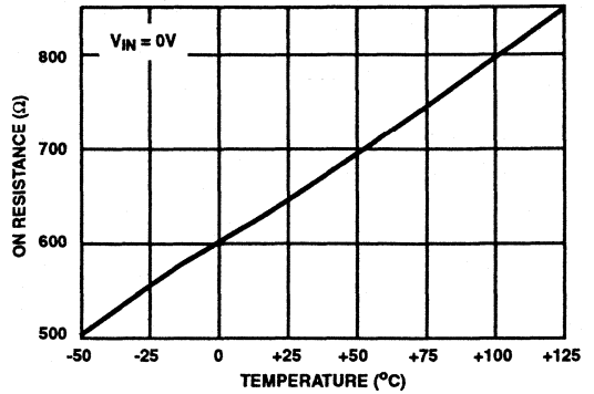
FIGURE 1B. ON RESISTANCE vs TEMPERATURE
