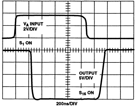
FIGURE 8D. ACCESS TIME
