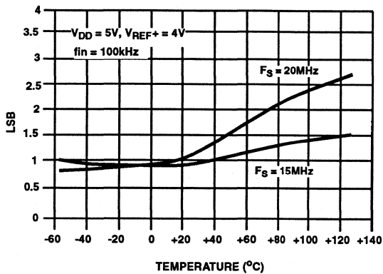
FIGURE 7. INL vs TEMPERATURE
