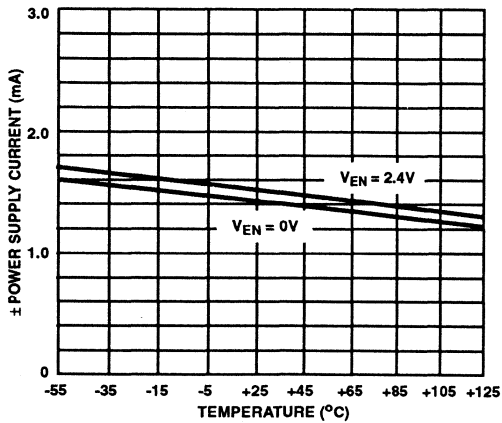
FIGURE 5A. HI-506/HI-507
