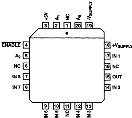
HI-1818A (PLCC) TOP VIEW
