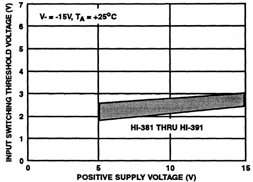
FIGURE 13. INPUT SWITCHING THRESHOLD vs POSITIVE SUPPLY VOLTAGE, HI-381 THRU HI-390
