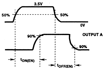
FIGURE 7A. ENABLE DRIVE
