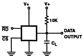
FIGURE 1C. t_{OH}
