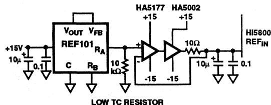
FIGURE 6. EXTERNAL REFERENCE
