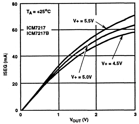
FIGURE 5. TYPICAL ISEG vs V_{OUT}
