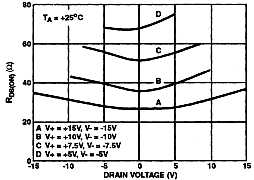
FIGURE 2. R_{DS(ON)} vs V_D AND POWER SUPPLY VOLTAGE
