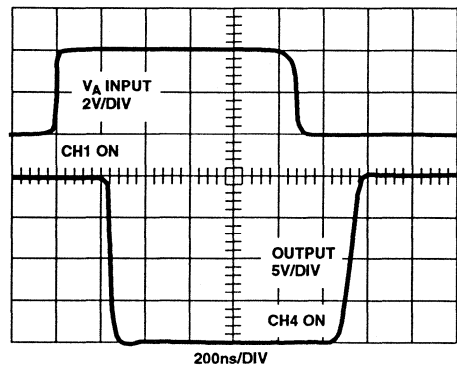
FIGURE 4D. ACCESS TIME WAVEFORMS
