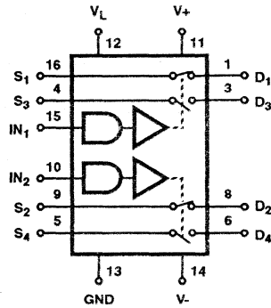
DIP (JE, PE) DUAL SPDT IH5143
