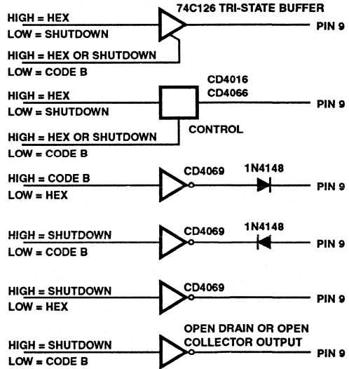
FIGURE 17. ICM7228C/D PIN 9 DRIVE CIRCUITS
