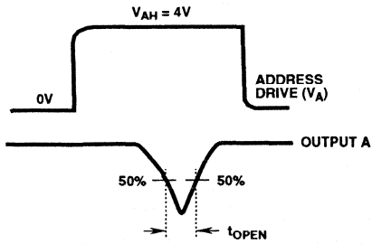
FIGURE 5A. t_{\text{OPEN}} MEASUREMENT
