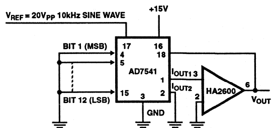
FIGURE 8. FEEDTHROUGH ERROR TEST CIRCUIT
