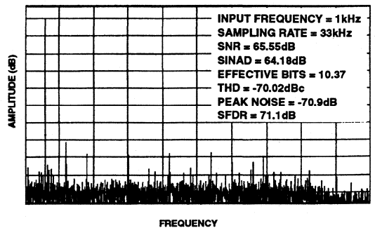
FIGURE 5. FFT SPECTRUM
