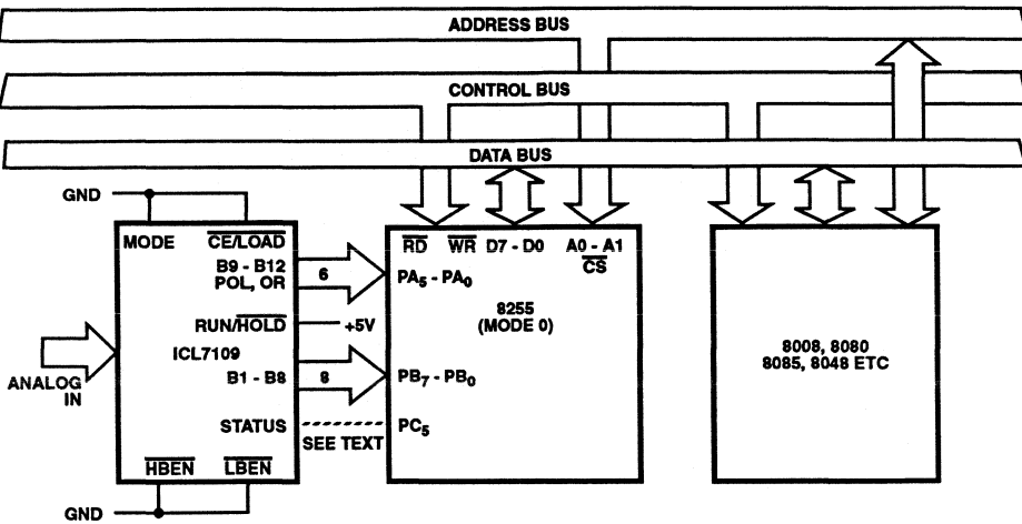
FIGURE 14. FULL-TIME PARALLEL INTERFACE TO 8040/8080/85 MICROPROCESSORS
