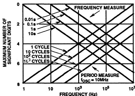
FIGURE 16. MAXIMUM ACCURACY OF FREQUENCY AND PERIOD MEASUREMENTS DUE TO LIMITATIONS OF QUANTIZATION ERRORS
