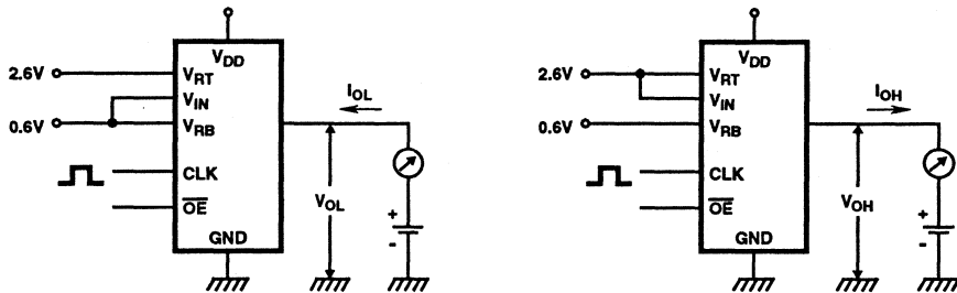
FIGURE 10. DIGITAL OUTPUT CURRENT TEST CIRCUIT
