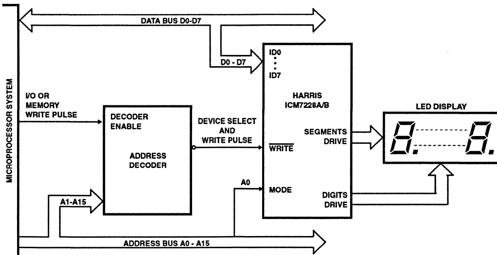
FIGURE 9. ICM7228A/B MICROPROCESSOR SYSTEM INTERFACING
