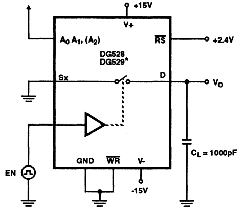
FIGURE 8B. CHARGE INJECTION TEST CIRCUIT * Similar connections for DG526, DG527
