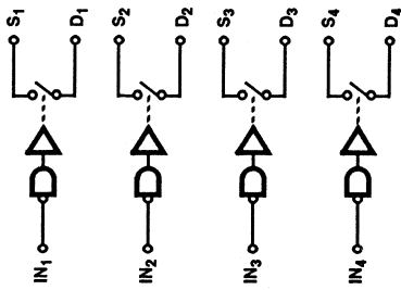
FIGURE 3. QUAD SPST
