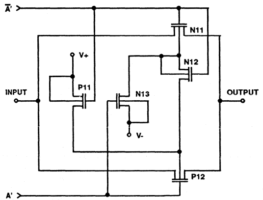
SWITCH CELL
