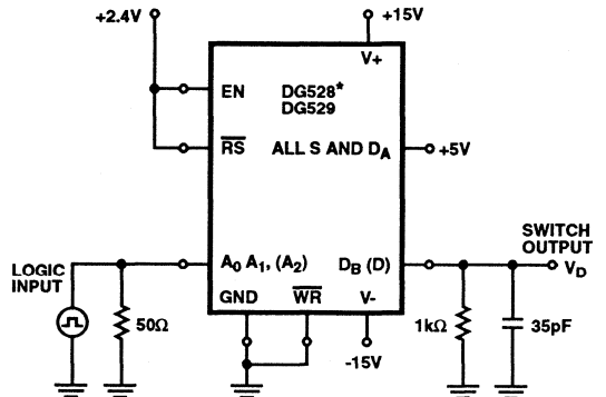
FIGURE 4B. t_{\text{OPEN}} (BREAK-BEFORE-MAKE) SWITCHING TIME TEST CIRCUIT
