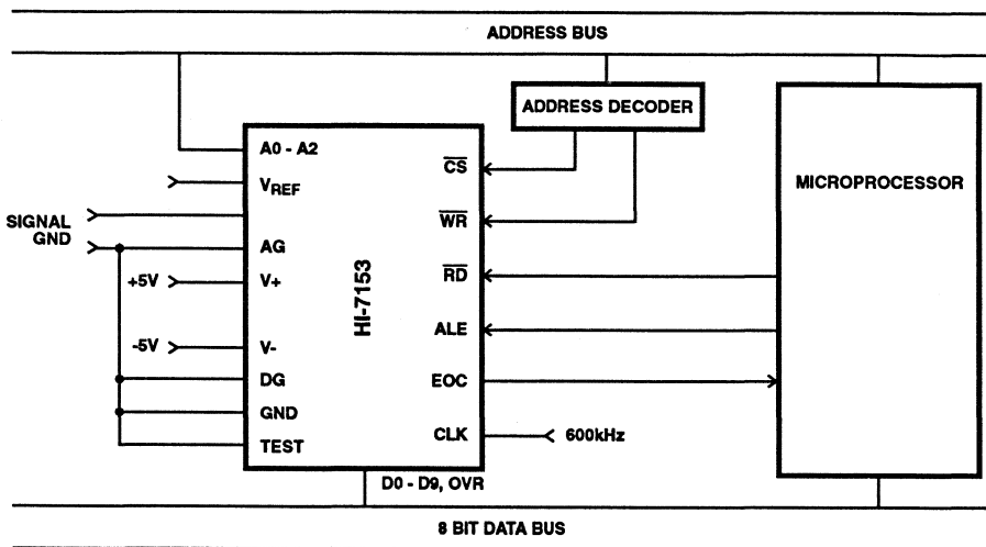
FIGURE 4. MULTI-CHANNEL DATA ACQUISITION SYSTEM
