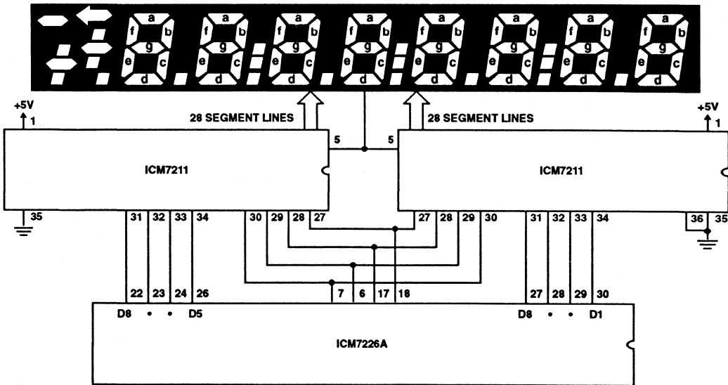
FIGURE 26. 10MHz UNIVERSAL COUNTER SYSTEM WITH LCD DISPLAY
