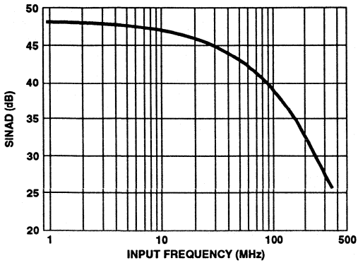
FIGURE 8. SINAD vs INPUT FREQUENCY CHARACTERISTICS
