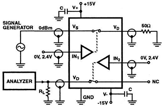
FIGURE 10. CROSSTALK
