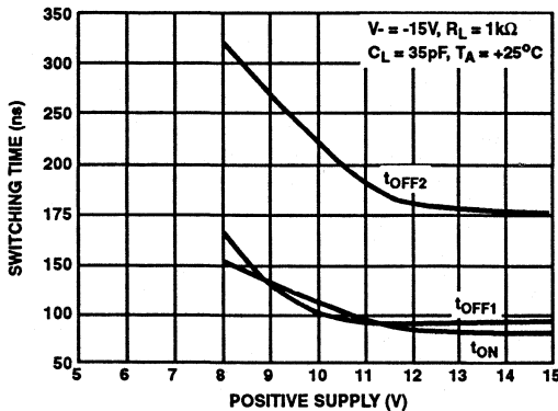
FIGURE 12. SWITCHING TIME vs POSITIVE SUPPLY VOLTAGE
