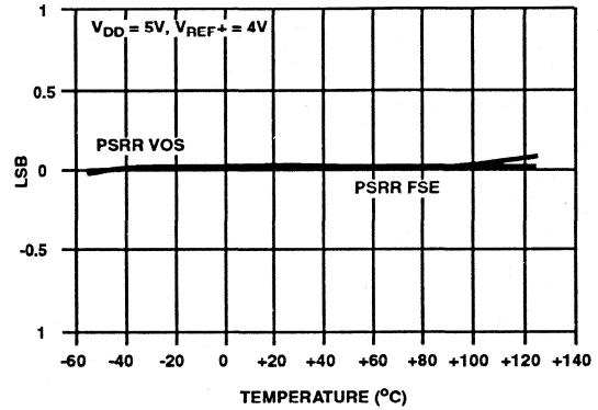
FIGURE 12. POWER SUPPLY REJECTION vs. TEMPERATURE
