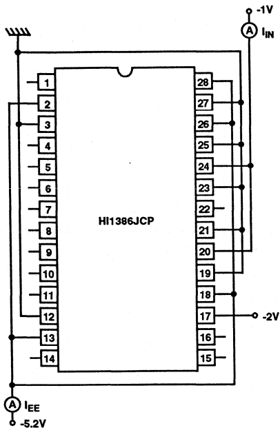
FIGURE 5A. FIGURE 5. ANALOG INPUT BIAS AND POWER SUPPLY CURRENT TEST CIRCUITS
