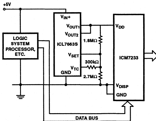
FIGURE 12. FLEXIBLE TEMPERATURE COMPENSATION
