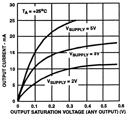
FIGURE 5. OUTPUT CURRENT AS A FUNCTION OF OUTPUT SATURATION VOLTAGE
