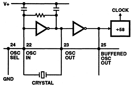
FIGURE 11. CRYSTAL OSCILLATOR
