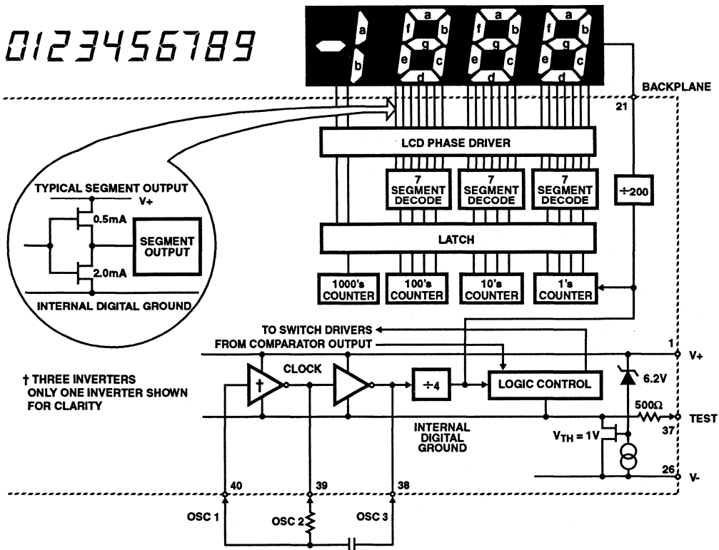
FIGURE 7. ICL7136 DIGITAL SECTION
