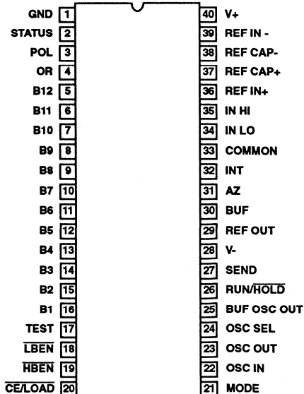
ICL7109 (CDIP, PDIP) TOP VIEW
