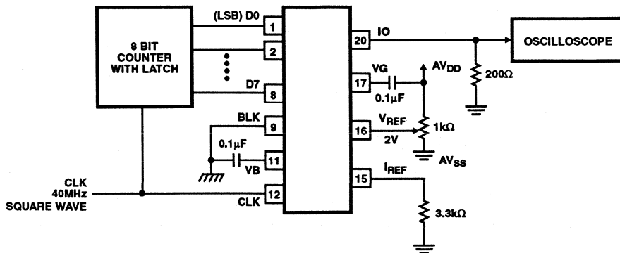
FIGURE 7. MAXIMUM CONVERSION SPEED TEST CIRCUIT
