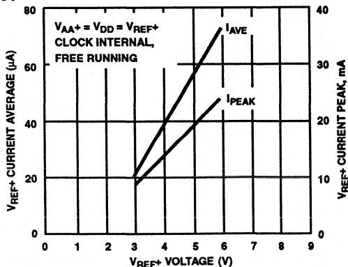
FIGURE 10. V_{REF+} CURRENT vs V_{REF+} VOLTAGE
