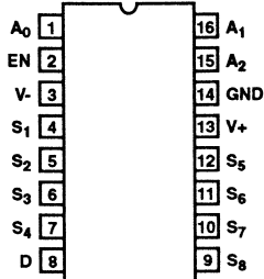
DG458 (CDIP, PDIP, SOIC) TOP VIEW
