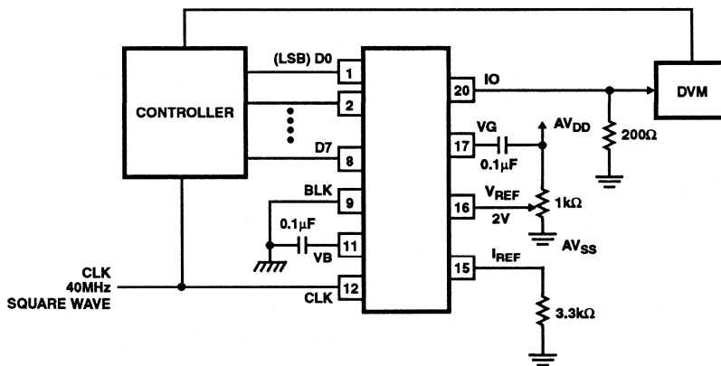
FIGURE 8. DC CHARACTERISTICS TEST CIRCUIT
