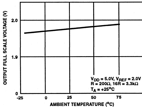
FIGURE 6. OUTPUT FULL SCALE VOLTAGE vs AMBIENT TEMPERATURE
