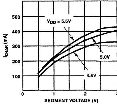
FIGURE 5. CHARACTER CURRENT VS OUTPUT VOLTAGE
