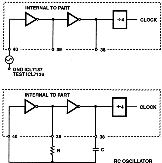
FIGURE 9. CLOCK CIRCUITS
