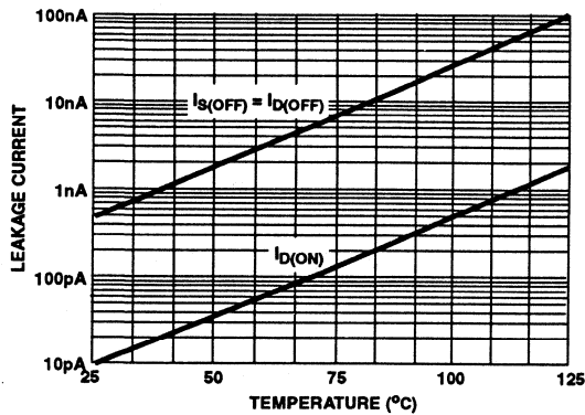
FIGURE 6. ON/OFF LEAKAGE CURRENT vs TEMPERATURE
