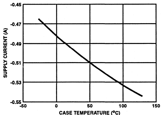
FIGURE 3. SUPPLY CURRENT vs TEMPERATURE CHARACTERISTICS
