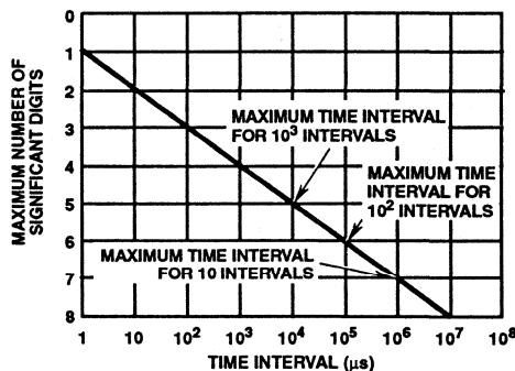
FIGURE 17. MAXIMUM ACCURACY OF TIME INTERVAL MEASUREMENT DUE TO LIMITATIONS OF QUANTIZATION ERRORS
