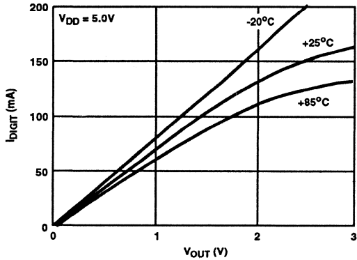
FIGURE 6. ICM7216B & ICM7216D TYPICAL I_{DIGIT} vs V_{OUT}
