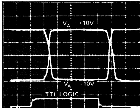
FIGURE 18. +25°C TTL OPEN COLLECTOR LOGIC DRIVE (Corresponds to Figure 19)
