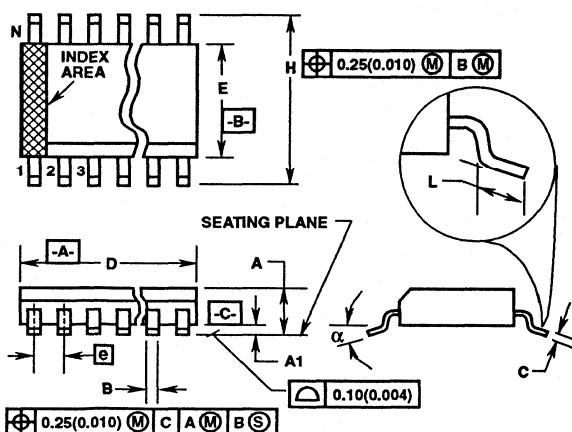
M28.209 (JEDEC MO-150-AH ISSUE A) 28 LEAD SHRINK SMALL OUTLINE PLASTIC PACKAGE
