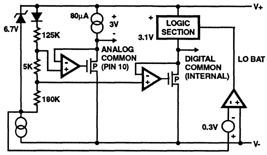
FIGURE 10. ANALOG AND DIGITAL COMMON VOLTAGE GENERATOR CIRCUIT
