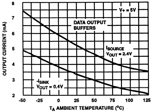
FIGURE 8. OUTPUT CURRENT vs TEMPERATURE
