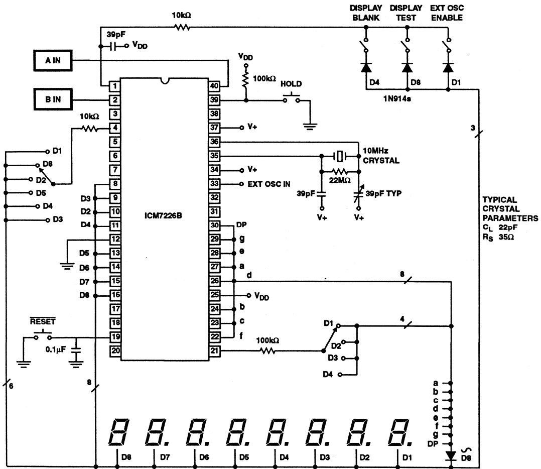
FIGURE 20. 10MHz UNIVERSAL COUNTER
