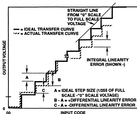
FIGURE 4. D/A INTEGRAL AND DIFFERENTIAL LINEARITY ERROR
