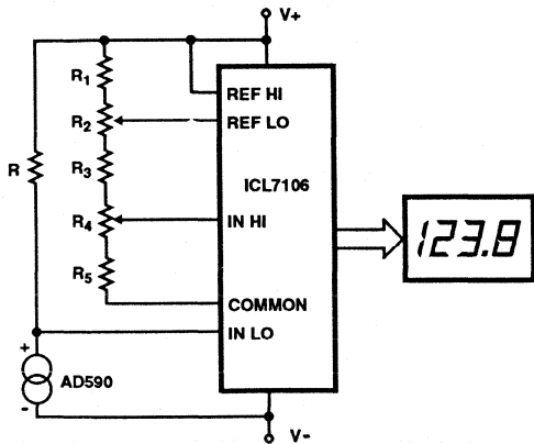
FIGURE 11. BASIC DIGITAL THERMOMETER, CELSIUS AND FAHRENHEIT SCALES
