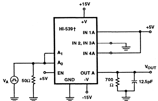
FIGURE 5B. t_{\text{OPEN}} TEST CIRCUIT
