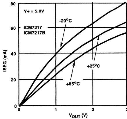
FIGURE 6. TYPICAL ISEG vs V_{OUT}
