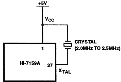
FIGURE 7. SINGLE-PIN OSCILLATOR
