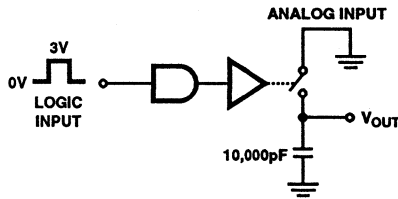
FIGURE 5. CHARGE INJECTION TEST CIRCUIT
