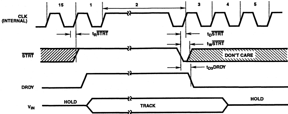
FIGURE 3. SINGLE SHOT MODE INTERNAL CLOCK
