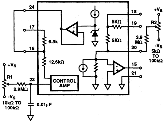
FIGURE 2. HI-DAC80V/HI-DAC85V
