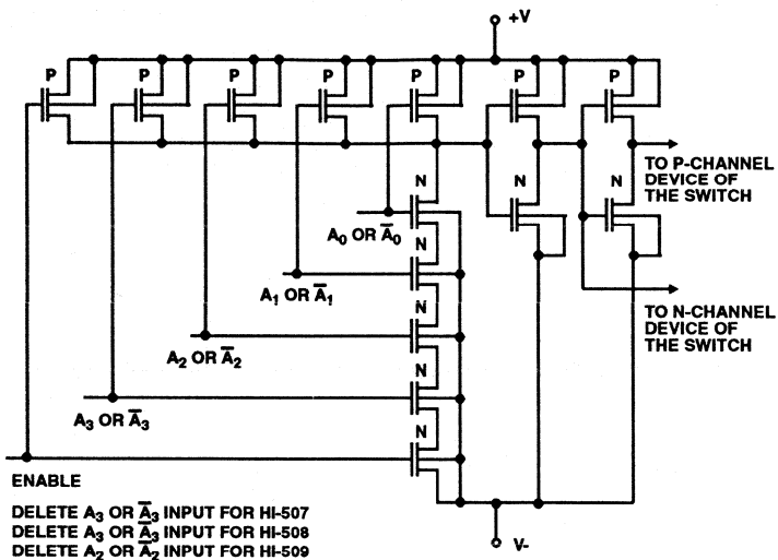
ADDRESS DECODER
