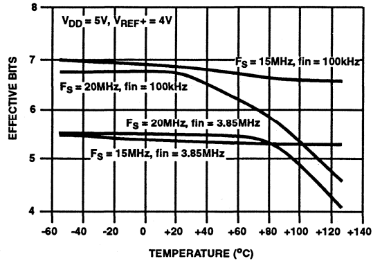
FIGURE 4. EFFECTIVE NUMBER OF BITS vs TEMPERATURE
