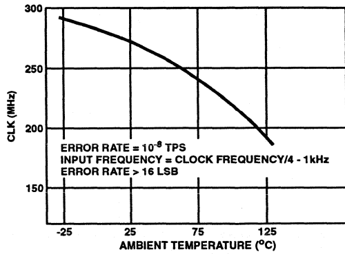
FIGURE 13. MAXIMUM CONVERSION RATE vs TEMPERATURE CHARACTERISTICS
