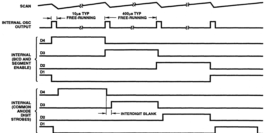
FIGURE 1. MULTIPLEX TIMING
