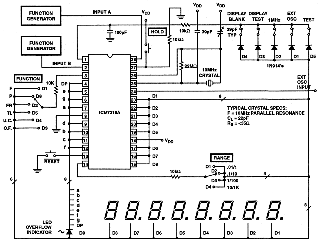
FIGURE 17. TEST CIRCUIT (ICM7216A SHOWN, OTHERS SIMILAR)
