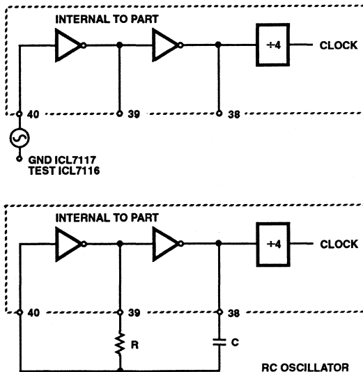
FIGURE 9. CLOCK CIRCUITS
