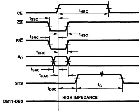
FIGURE 4. CONVERT START TIMING
