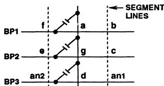
FIGURE 6. DISPLAY SCHEMATIC
