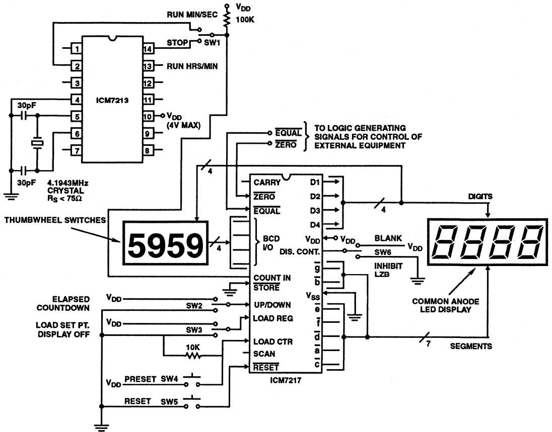
FIGURE 21. PRECISIONS TIMER
