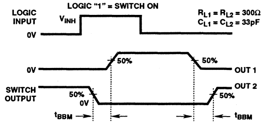
FIGURE 18. BREAK-BEFORE-MAKE TEST CIRCUIT ( t_{BBM} )
