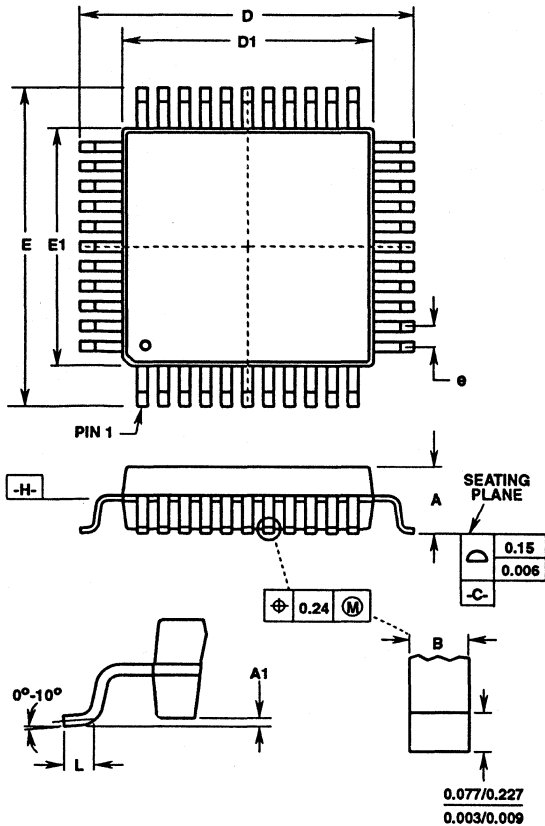
Q32.A 32 LEAD METRIC PLASTIC QUAD FLATPACK PACKAGE
