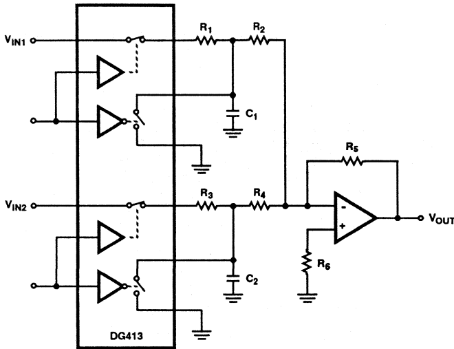
FIGURE 13. SUMMING AMPLIFIER
