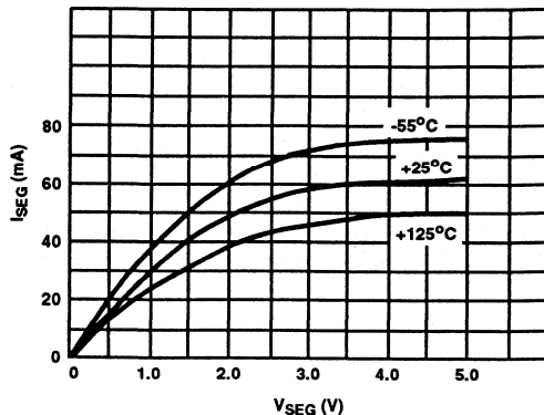
FIGURE 6. COMMON ANODE SEGMENT DRIVER I_{SEG} vs V_{SEG}
