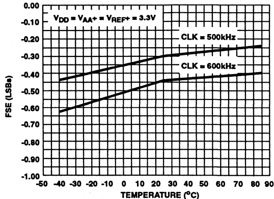
FIGURE 9. FULL SCALE ERROR vs TEMPERATURE
