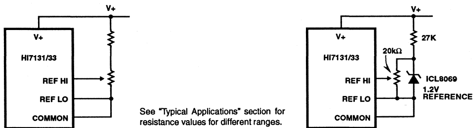
FIGURE 11. HI7131 TYPICAL REFERENCE CIRCUITS
