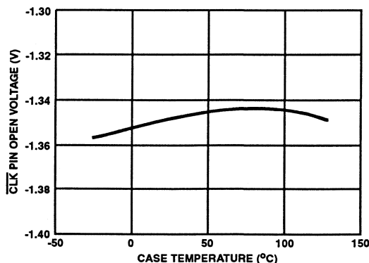
FIGURE 7. CLK PIN OPEN VOLTAGE vs TEMPERATURE CHARACTERISTICS
