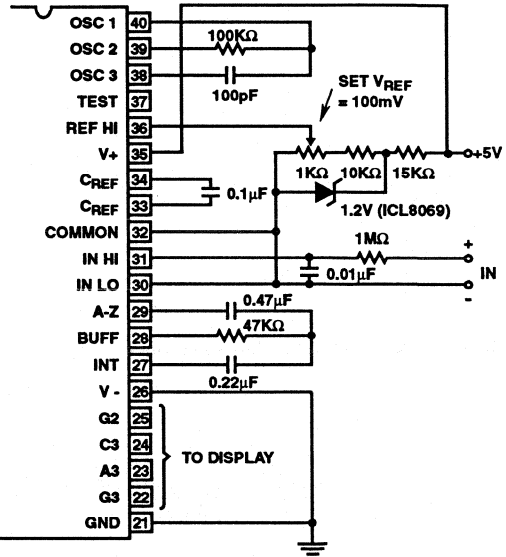
FIGURE 14. ICL7117 OPERATED FROM SINGLE +5V SUPPLY
