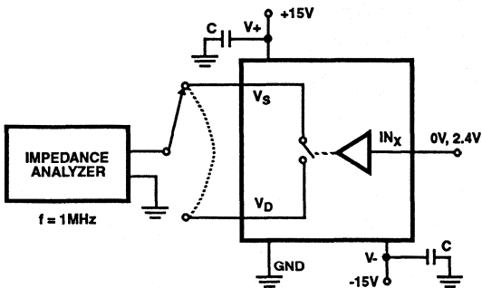
FIGURE 22. SOURCE/DRAIN CAPACITANCES
