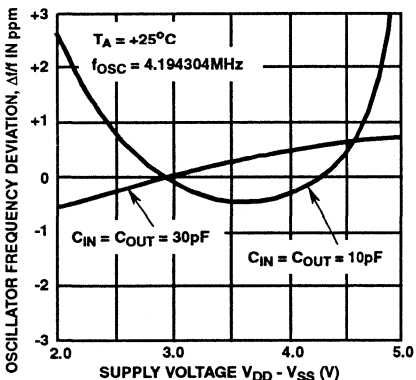
FIGURE 7. OSCILLATOR STABILITY AS A FUNCTION OF SUPPLY VOLTAGE
