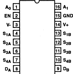
DG459 (CDIP, PDIP, SOIC) TOP VIEW
