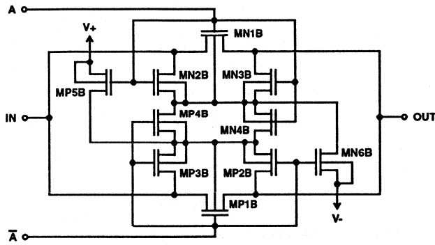
SWITCH CELL
