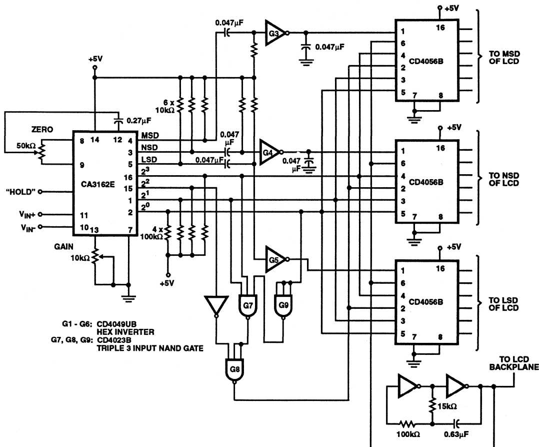
FIGURE 3. TYPICAL LCD APPLICATION
