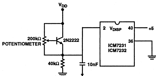
FIGURE 11B. TRANSISTOR-MULTIPLIER
