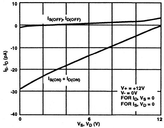
FIGURE 14. SOURCE/DRAIN LEAKAGE CURRENTS (SINGLE 12V SUPPLY)
