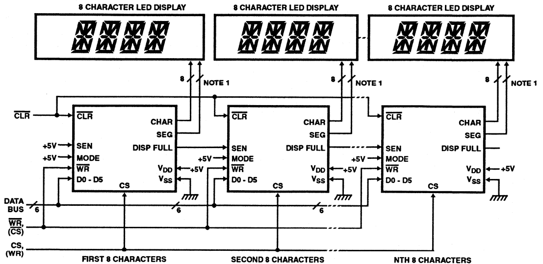
FIGURE 8. MULTICHARACTER DISPLAY USING SEQUENTIAL ACCESS MODE
