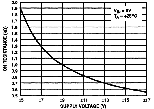
FIGURE 1D. ON RESISTANCE vs SUPPLY VOLTAGE
