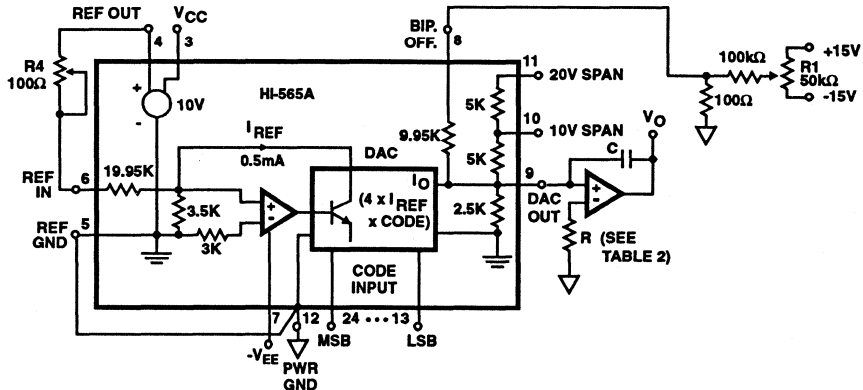
FIGURE 1. UNIPOLAR VOLTAGE OUTPUT
