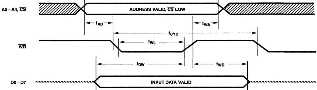
FIGURE 2. WRITE CYCLE TIMING FOR NON-MULTIPLEXED BUS ( ALE = V_{IH} , \overline{RD} = V_{IH} )
