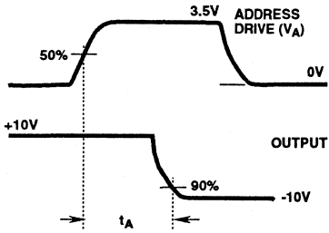
FIGURE 8C. WAVEFORMS
