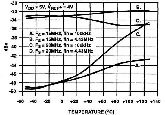
FIGURE 6. TOTAL HARMONIC DISTORTION vs TEMPERATURE
