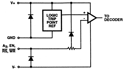
LOGIC INTERFACE AND LEVEL SHIFTER
