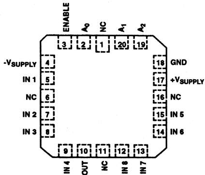
HI-508 (LCC, PLCC) TOP VIEW
