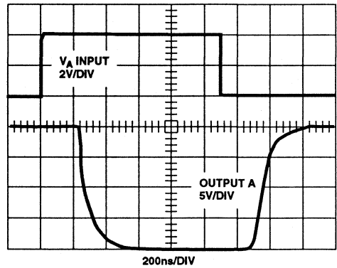
FIGURE 7B. ACCESS TIME WAVEFORMS
