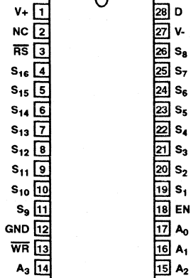
DG526 (PDIP, SOIC) TOP VIEW
