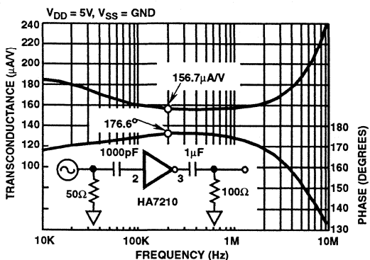
FIGURE 37. TRANSCONDUCTANCE vs FREQUENCY F1 = 1, F2 = 0
