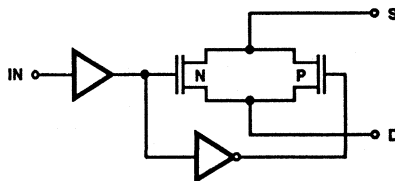
TYPICAL SWITCH HI-300 SERIES
