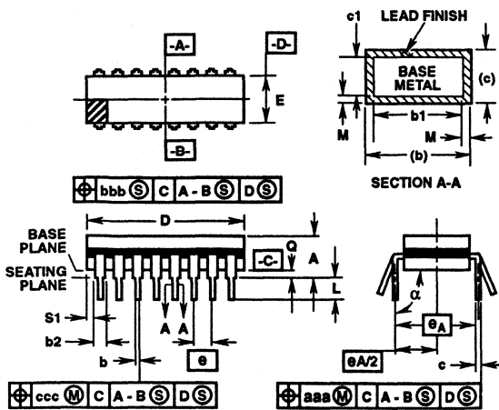
F40.6 MIL-STD-1835 GDIP1-T40 (D-5, CONFIGURATION A) 40 LEAD DUAL-IN-LINE FRIT-SEAL CERAMIC PACKAGE
