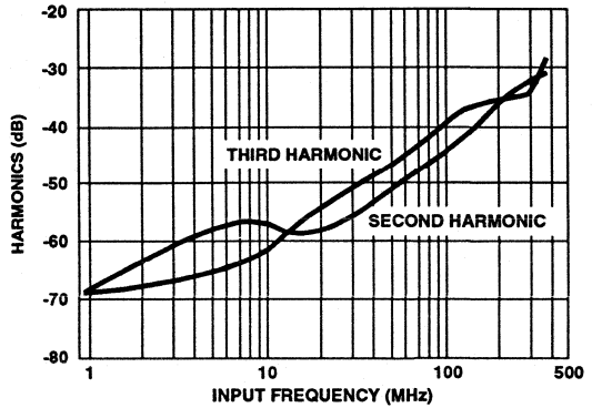
FIGURE 9. HARMONIC DISTORTION vs INPUT FREQUENCY CHARACTERISTICS
