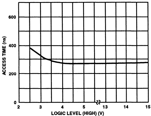
FIGURE 8A. ACCESS TIME vs LOGIC LEVEL (HIGH)
