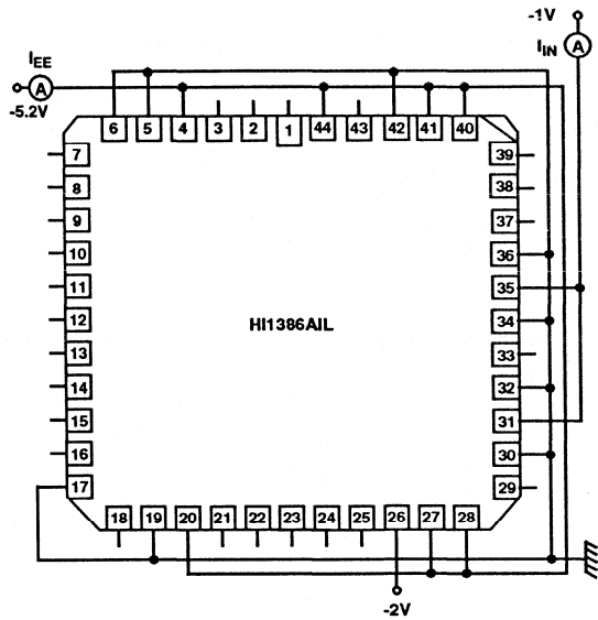
FIGURE 5A. FIGURE 5. ANALOG INPUT BIAS AND POWER SUPPLY CURRENT TEST CIRCUITS
