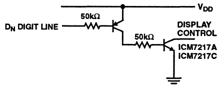
FIGURE 12B. COMMON CATHODE
