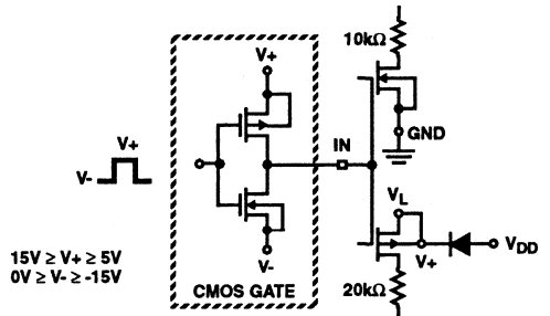
FIGURE 14. INTERFACING WITH CMOS LOGIC
