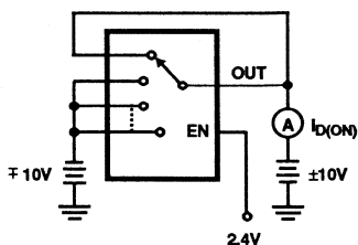
FIGURE 4. I_{D(ON)} (NOTE 1)
