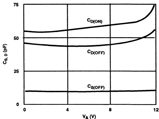
FIGURE 2. SOURCE/DRAIN CAPACITANCE vs ANALOG VOLTAGE (SINGLE 12V SUPPLY)
