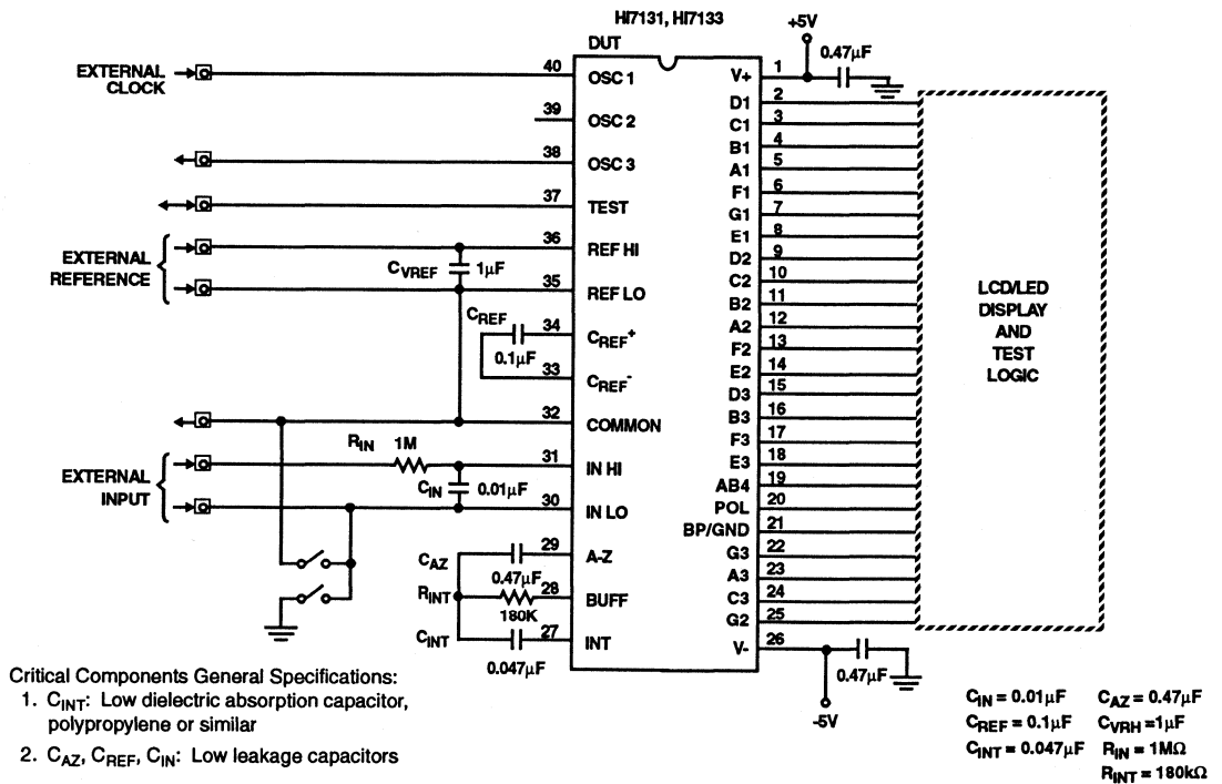
FIGURE 2. TEST CIRCUIT
