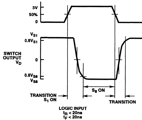
FIGURE 3C. t_{\text{TRANSITION}} SWITCHING TIME WAVEFORM
