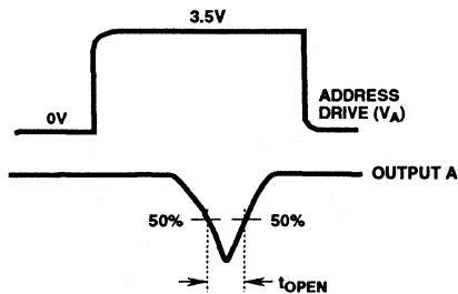
FIGURE 6A. ENABLE DRIVE
