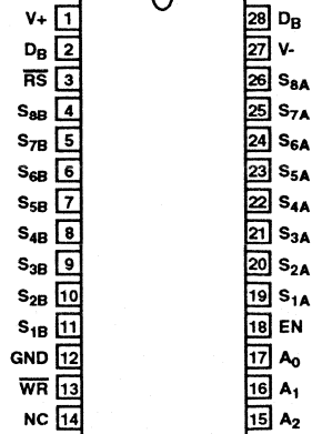
DG527 (PDIP, SOIC) TOP VIEW
