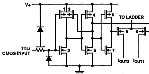
FIGURE 1. CMOS SWITCH
