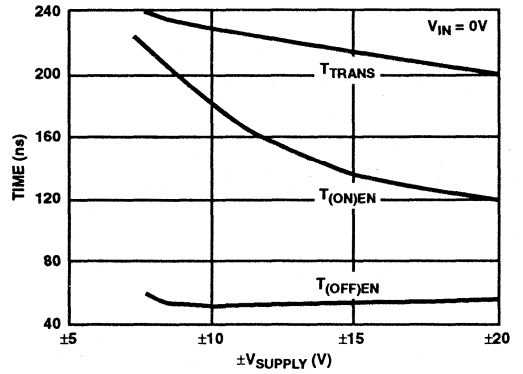
FIGURE 8. SWITCHING TIMES ( t_{TRANS} , t_{ON} , t_{OFF} ) vs \pm V SUPPLIES
