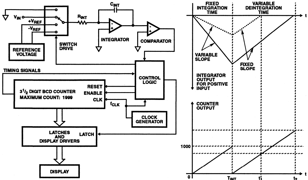
FIGURE 3. DUAL SLOPE INTEGRATING A/D CONVERTER
