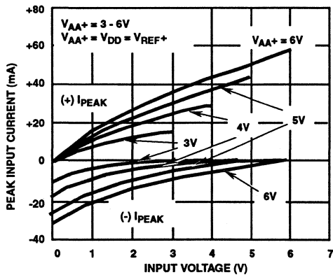
FIGURE 8. PEAK INPUT CURRENT vs INPUT VOLTAGE
