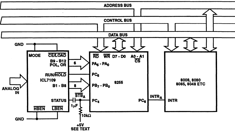
FIGURE 15. FULL-TIME PARALLEL INTERFACE TO 8048/8080/85 MICROPROCESSORS WITH INTERRUPT
