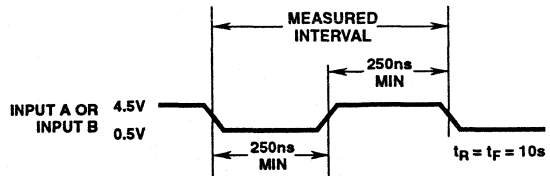
FIGURE 10. WAVEFORM FOR GUARANTEED MINIMUM f_B(\text{MAX}) AND f_A(\text{MAX}) FOR FUNCTION = PERIOD AND TIME INTERVAL
