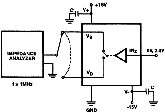
FIGURE 22. SOURCE/DRAIN CAPACITANCES
