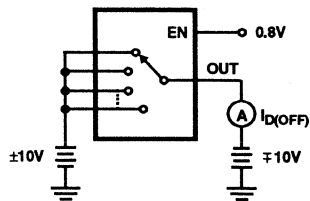
FIGURE 2. I_{D(OFF)} (NOTE 1)
