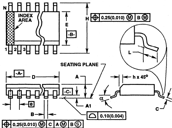
M16.3 (JEDEC MS-013-AA ISSUE C) 16 LEAD WIDE BODY SMALL OUTLINE PLASTIC PACKAGE
