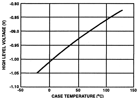
FIGURE 4. DO PIN HIGH LEVEL VOLTAGE vs TEMPERATURE CHARACTERISTICS
