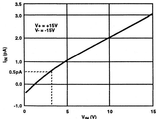
FIGURE 1. INPUT LOGIC CURRENT vs LOGIC INPUT VOLTAGE
