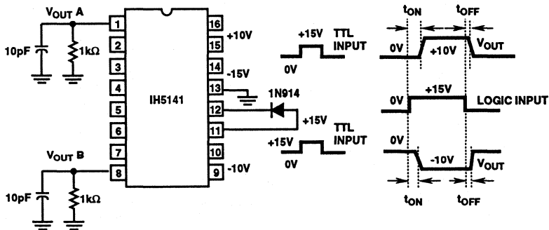
FIGURE 8. IH5141 t_{ON} AND t_{OFF} (15V DIGITAL INPUT)
