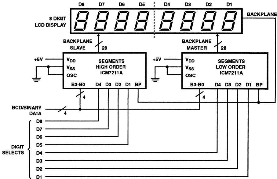
FIGURE 12. GANGED ICM7211's DRIVING 8-DIGIT LCD DISPLAY
