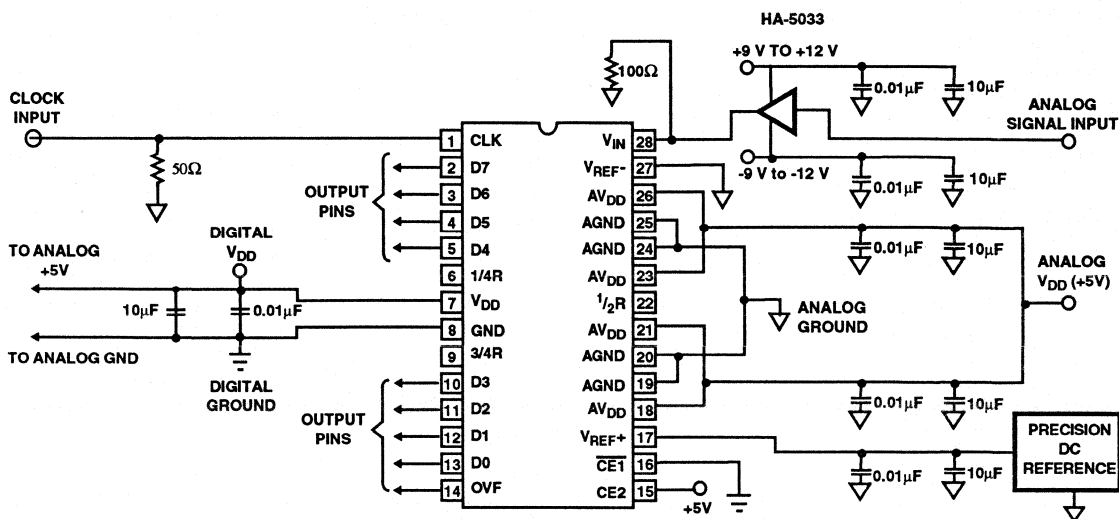
FIGURE 15. TEST CIRCUIT
