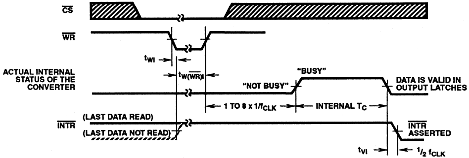
FIGURE 10A. START CONVERSION
