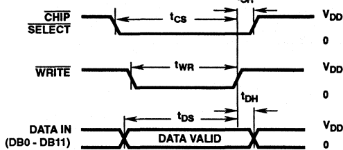
FIGURE 1B. PREFERRED WRITE CYCLE
