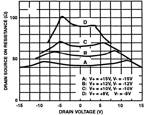
FIGURE 2. r_{DS(ON)} vs V_D AND POWER SUPPLY VOLTAGE
