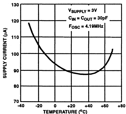
FIGURE 3. SUPPLY CURRENT AS A FUNCTION OF TEMPERATURE
