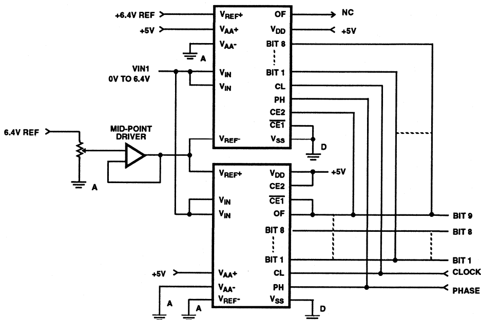
FIGURE 13. USING TWO CA3318s FOR 9-BIT RESOLUTION
