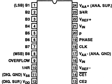
CA3318C (PDIP, CDIP, SOIC) TOP VIEW
