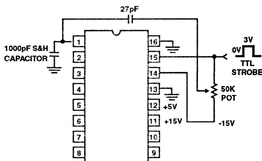
FIGURE 7. ADJUSTABLE CHARGE INJECTION COMPENSATION CIRCUIT
