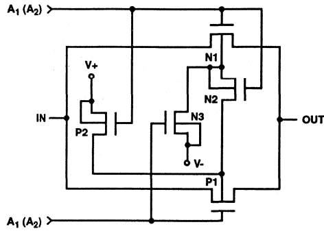
FIGURE 15. SWITCH CELL
