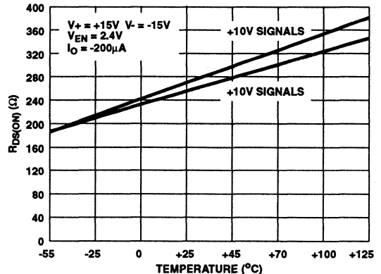
FIGURE 10. TYPICAL R_{DS(ON)} VARIATION WITH TEMPERATURE
