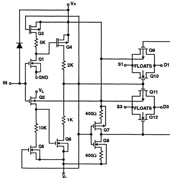
FUNCTIONAL DRIVER, TYPICAL DRIVER, GATE (1/2 AS SHOWN)
