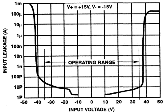
FIGURE 2. OFF CHANNEL LEAKAGE CURRENT vs INPUT VOLTAGE
