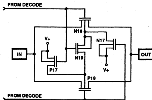
MULTIPLEXER SWITCH
