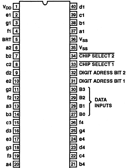
ICM7212AM (PDIP) TOP VIEW
