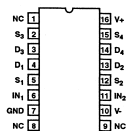
DG303ACY (SOIC) TOP VIEW
