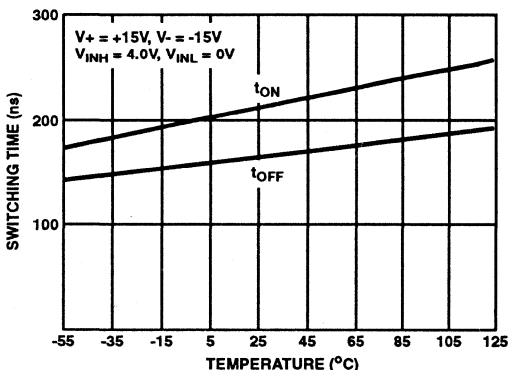
FIGURE 10. SWITCHING TIME vs TEMPERATURE, HI-300 THRU HI-303
