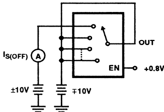
FIGURE 3. I_{S(OFF)} (NOTE 1)
