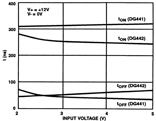
FIGURE 16. SWITCHING TIMES vs INPUT VOLTAGE
