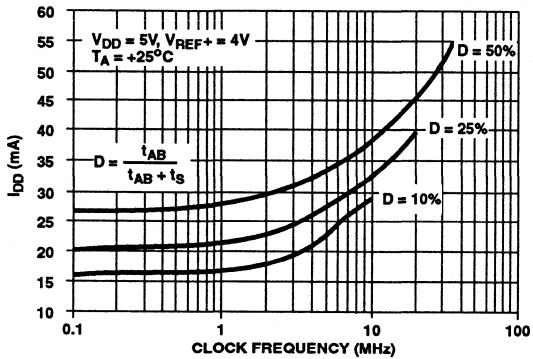
FIGURE 11. SUPPLY CURRENT vs CLOCK AND DUTY CYCLE
