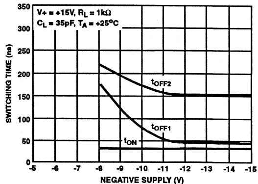
FIGURE 13. SWITCHING TIME vs NEGATIVE SUPPLY VOLTAGE
