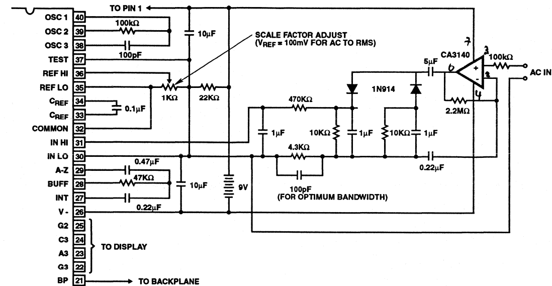
FIGURE 21. AC TO DC CONVERTER WITH ICL7106
