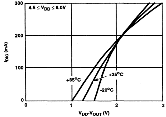
FIGURE 3. ICM7226A TYPICAL I_{DIG} vs V_{DD} - V_{OUT}
