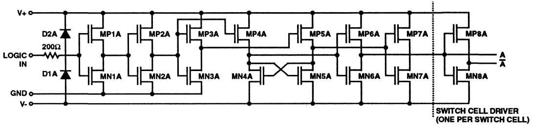
DIGITAL INPUT BUFFER AND LEVEL SHIFTER
