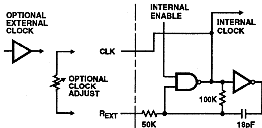
FIGURE 16. CLOCK CIRCUITRY
