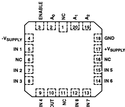
HI4P0548 (PLCC) TOP VIEW
