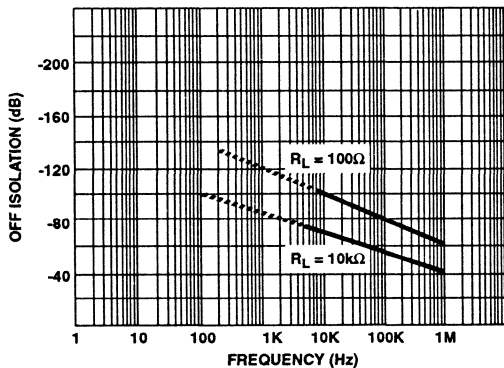
FIGURE 8. "OFF" ISOLATION vs FREQUENCY
