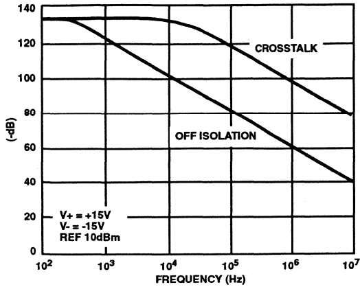
FIGURE 7. CROSSTALK AND OFF ISOLATION vs FREQUENCY
