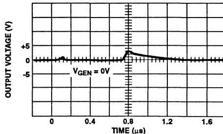
7F. V_{OUT} vs TIME
