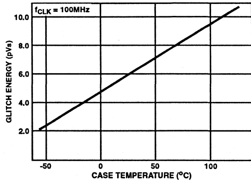
FIGURE 5. GLITCH ENERGY vs CASE TEMPERATURE (FULL SCALE - 1023mV)
