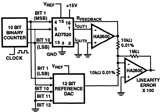
FIGURE 2. NONLINEARITY
