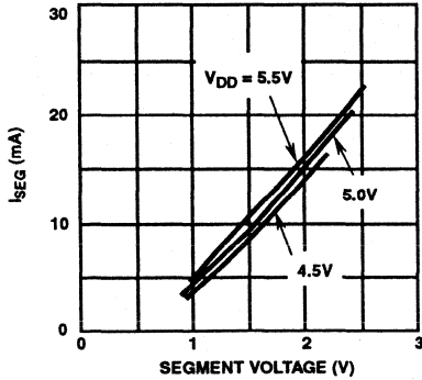
FIGURE 4. SEGMENT CURRENT vs OUTPUT VOLTAGE
