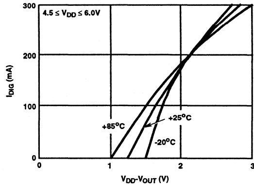
FIGURE 3. ICM7216A TYPICAL I_{DIG} vs V_{DD}-V_{OUT}
