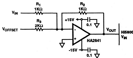
FIGURE 5. INVERTING BUFFER
