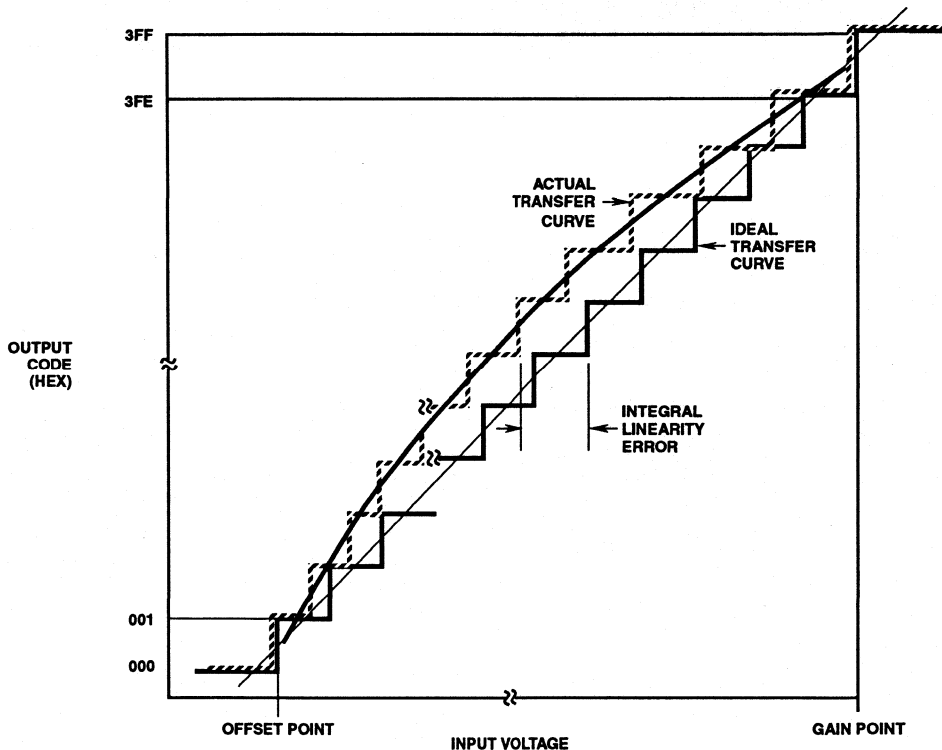
FIGURE 19. NORMALIZED GAIN, OFFSET, INTEGRAL AND DIFFERENTIAL LINEARITY ERRORS vs REFERENCE VOLTAGE
