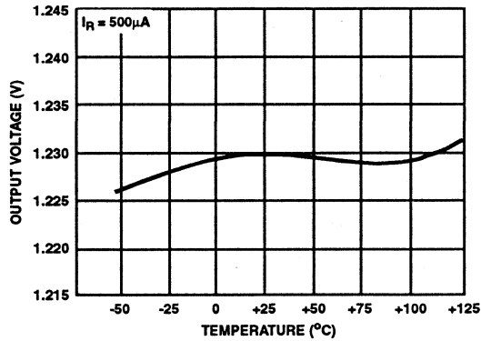
FIGURE 3. REVERSE VOLTAGE AS A FUNCTION OF TEMPERATURE
