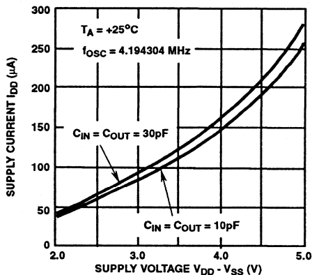
FIGURE 4. SUPPLY CURRENT AS A FUNCTION OF SUPPLY VOLTAGE
