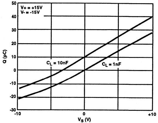
FIGURE 6. CHARGE INJECTION vs SOURCE VOLTAGE
