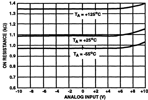
FIGURE 1B. ON RESISTANCE vs ANALOG INPUT VOLTAGE
