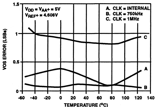
FIGURE 7. OFFSET VOLTAGE vs TEMPERATURE
