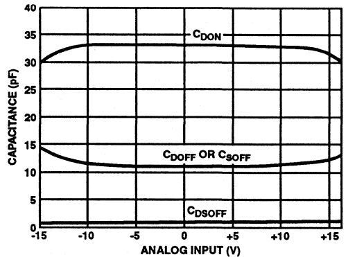
FIGURE 17. CAPACITANCE vs ANALOG INPUT
