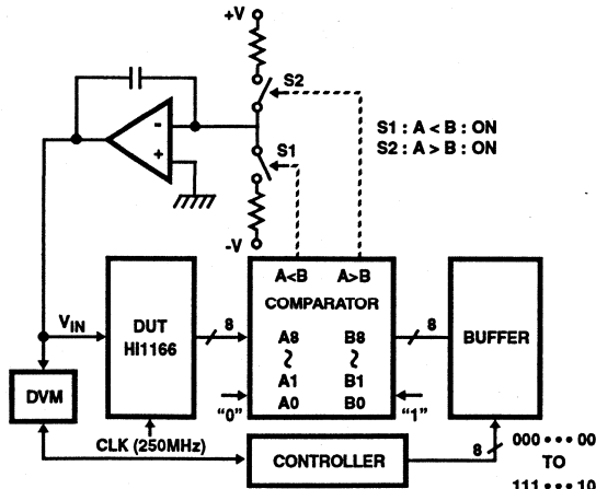
FIGURE 3. INTEGRAL AND DIFFERENTIAL LINEARITY ERROR TEST CIRCUIT
