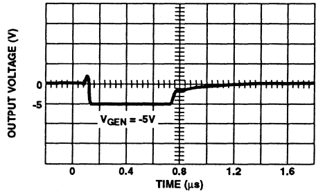
9F. V_{OUT} vs TIME
