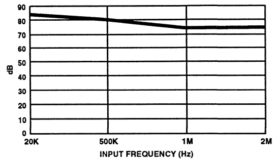
FIGURE 7. TYPICAL SFDR vs INPUT FREQUENCY
