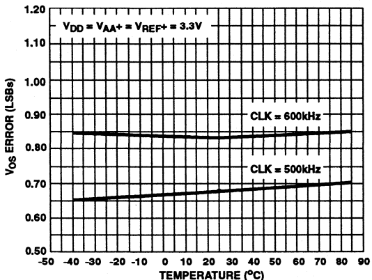
FIGURE 8. OFFSET ERROR vs TEMPERATURE
