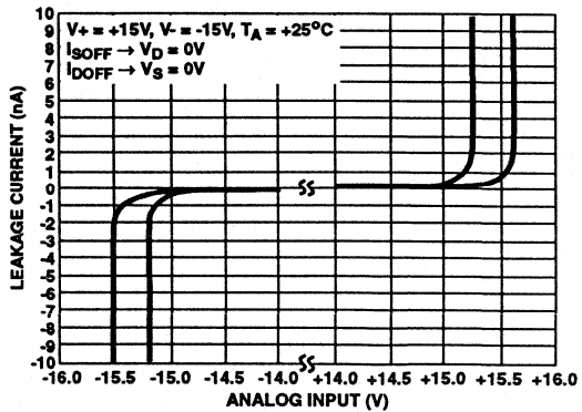
FIGURE 9. LEAKAGE CURRENT vs ANALOG INPUT VOLTAGE
