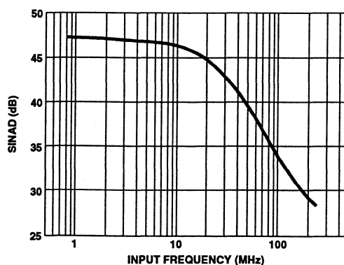
FIGURE 11. SINAD vs INPUT FREQUENCY RESPONSE CHARACTERISTICS
