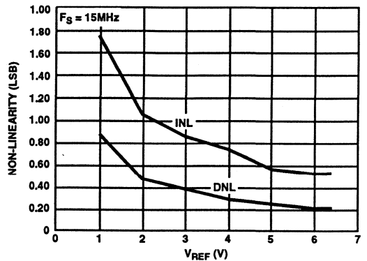
FIGURE 9. NON-LINEARITY vs REFERENCE VOLTAGE
