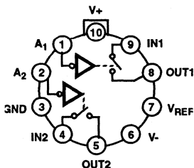
HI-200 (CAN) TOP VIEW
