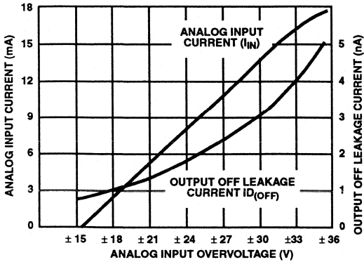
FIGURE 3A. ANALOG INPUT CURRENT AND OUTPUT OFF LEAKAGE CURRENT vs ANALOG INPUT OVERVOLTAGE
