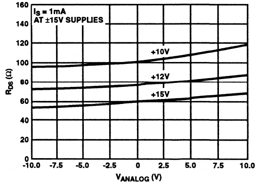
FIGURE 2. R_{DS(ON)} vs POWER SUPPLY VOLTAGE
