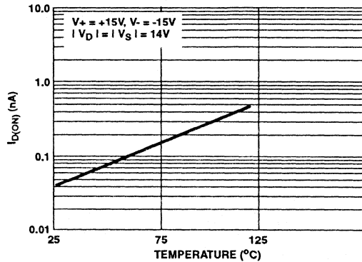
FIGURE 6. I_{D(ON)} vs TEMPERATURE*
