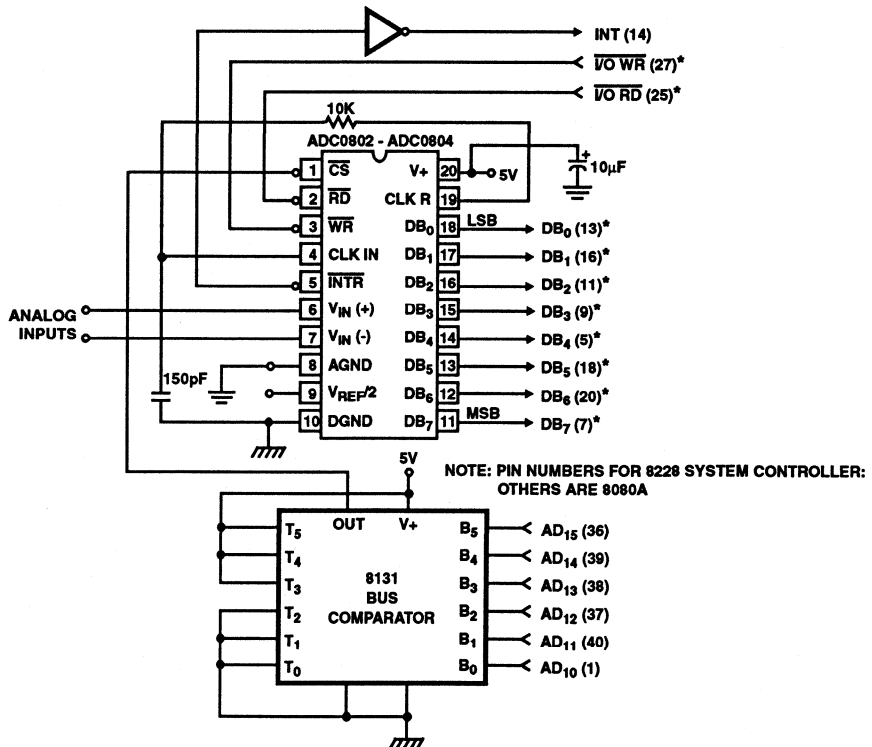
FIGURE 21. ADC0802 TO 8080A CPU INTERFACE
