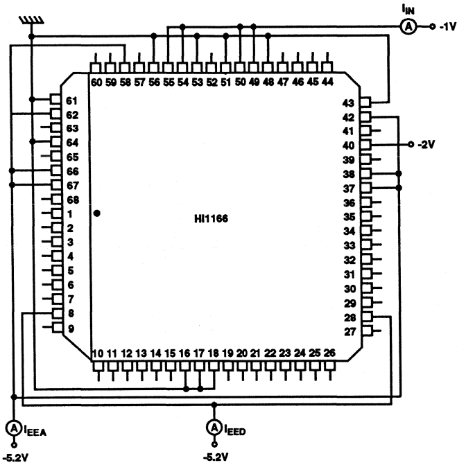
FIGURE 4. POWER SUPPLY AND ANALOG INPUT BIAS CURRENT TEST CIRCUIT
