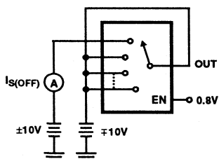
FIGURE 3. I_{S(OFF)} (NOTE 1)
