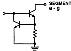
SEGMENT DRIVER
