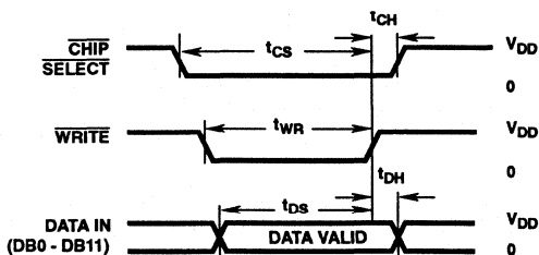
FIGURE 1A. TYPICAL WRITE CYCLE
