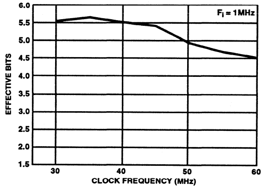
FIGURE 12. EFFECTIVE NUMBER OF BITS vs CLOCK FREQUENCY
