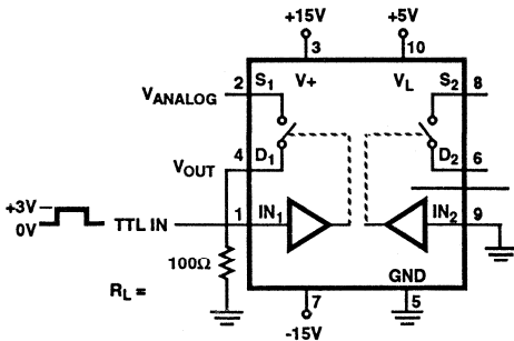
FIGURE 7A. SWITCHING TIME TEST CIRCUIT
