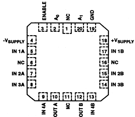
HI-509 (LCC, PLCC) TOP VIEW
