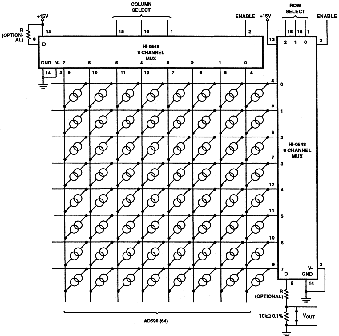
FIGURE 17. MULTIPLEXING SENSORS
