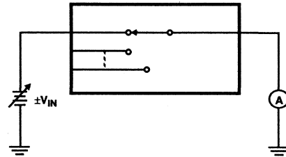
FIGURE 4B. ON CHANNEL CURRENT TEST CIRCUIT
