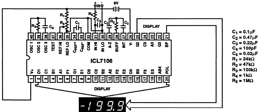
FIGURE 1. ICL7106 TEST CIRCUIT AND TYPICAL APPLICATION WITH LCD DISPLAY COMPONENTS SELECTED FOR 200mV FULL-SCALE
