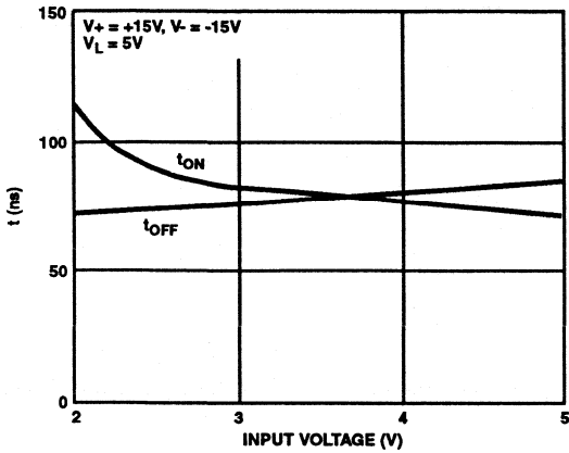
FIGURE 13. SWITCHING TIME vs INPUT VOLTAGE (DG445)
