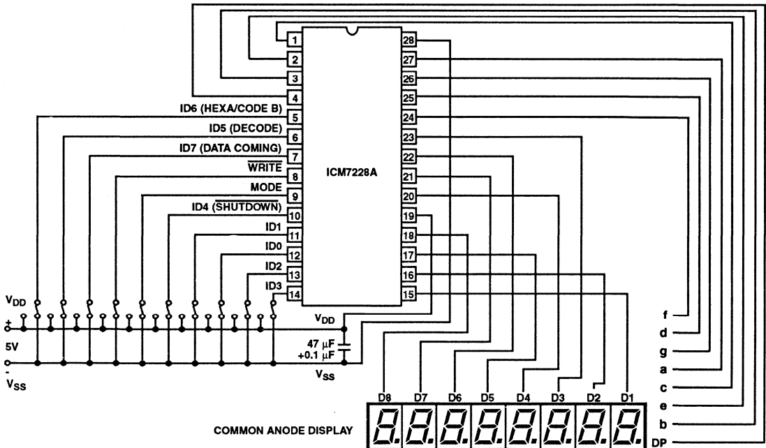
FIGURE 18. FUNCTIONAL TEST CIRCUIT #1
