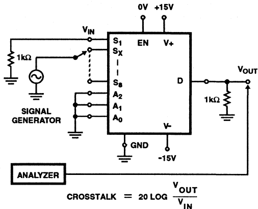
FIGURE 30. CROSSTALK
