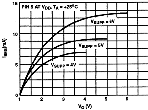
FIGURE 5. ICM7212 LED SEGMENT CURRENT AS A FUNCTION OF OUTPUT VOLTAGE
