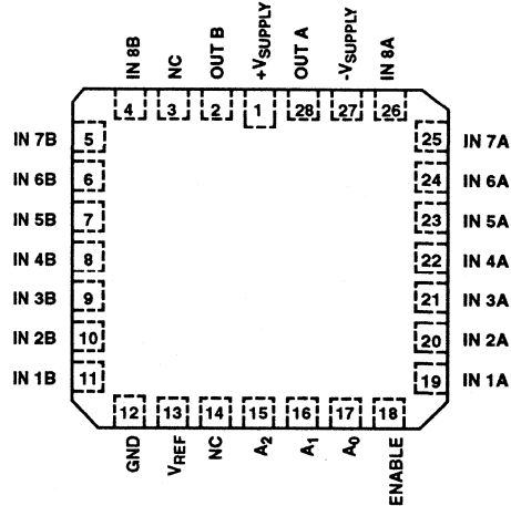
HI4P0547 (PLCC) TOP VIEW
