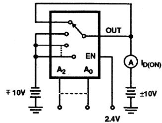
FIGURE 4. I_{D(ON)} (NOTE 1)
