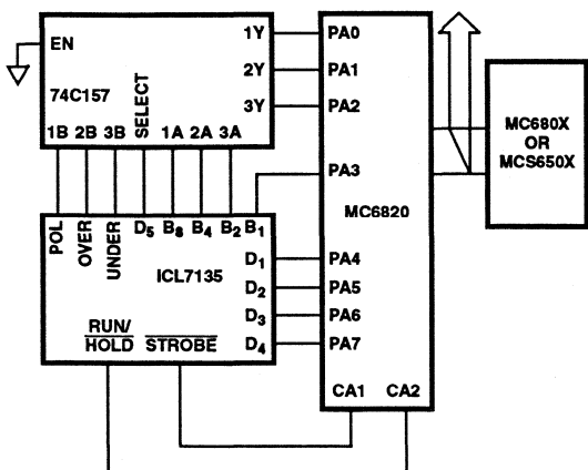
FIGURE 15. ICL7135 TO MC6800, MCS650X INTERFACED
