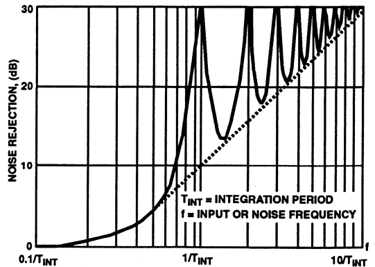
FIGURE 4. NOISE REJECTION FOR INTEGRATING TYPE A/D CONVERTER
