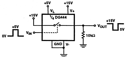
FIGURE 24. LEVEL SHIFTER
