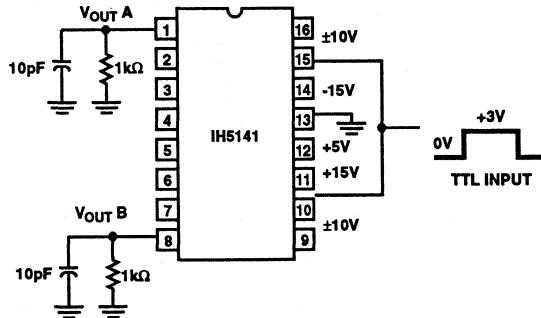
FIGURE 7. IH5141 t_{ON} AND t_{OFF} (3V DIGITAL INPUT)
