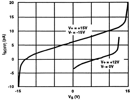
FIGURE 7. SOURCE LEAKAGE CURRENT vs SOURCE VOLTAGE
