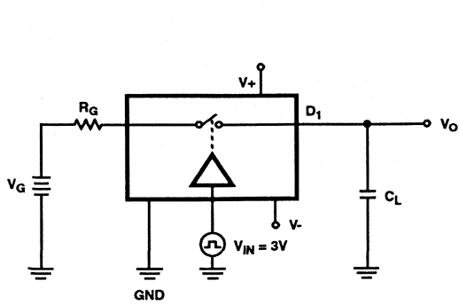
FIGURE 9. CHARGE INJECTION
