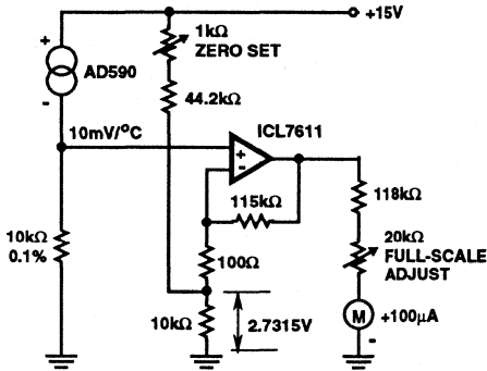
FIGURE 14. CENTIGRADE THERMOMETER (0°C - +100°C)
