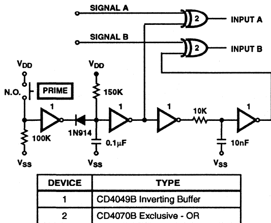
FIGURE 15. PRIMING CIRCUIT, SIGNALS A & B BOTH HIGH OR LOW
