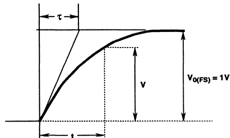
FIGURE 12. D/A OUTPUT WAVEFORM
