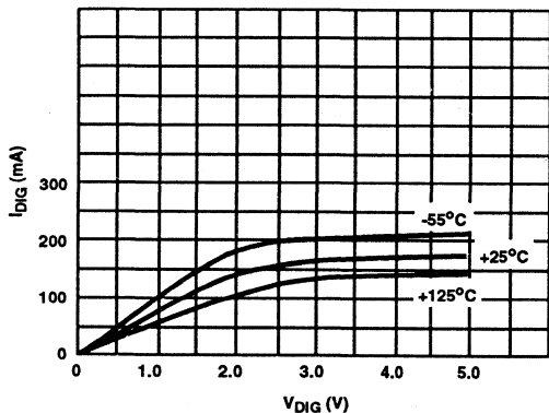
FIGURE 7. COMMON CATHODE DIGIT DRIVER I_{DIG} vs V_{DIG}
