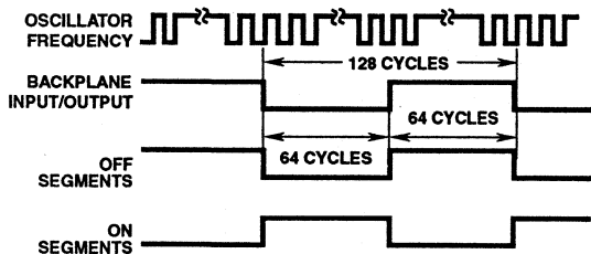
FIGURE 8. DISPLAY WAVEFORMS
