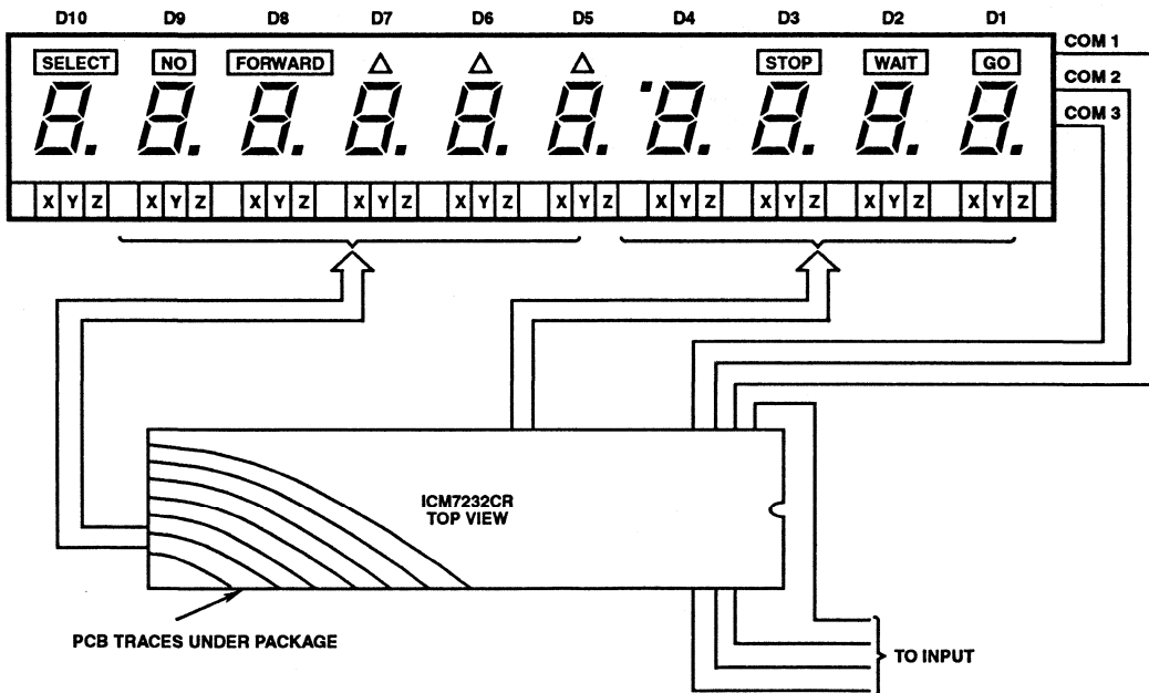
FIGURE 17. "REVERSE" PIN ORIENTATION AND DISPLAY CONNECTIONS
