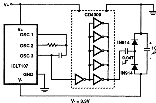
FIGURE 10. GENERATING NEGATIVE SUPPLY FROM +5V
