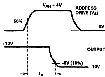
FIGURE 4C. ACCESS TIME MEASUREMENT
