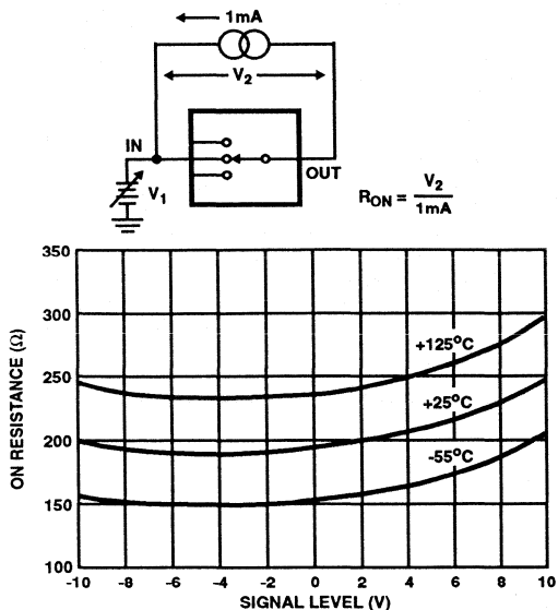
FIGURE 3. ON RESISTANCE vs ANALOG SIGNAL LEVEL
