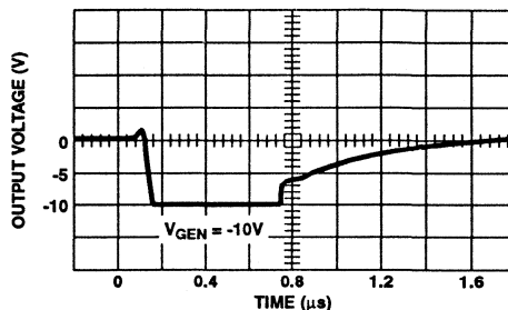
7H. V_{OUT} vs TIME
