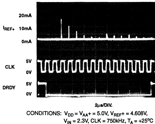
FIGURE 20. TYPICAL REFERENCE INPUT CURRENT
