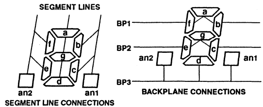
FIGURE 4. CONNECTION DIAGRAMS FOR TYPICAL 7-SEGMENT DISPLAYS
