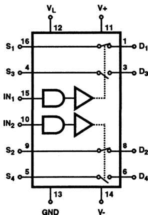
FIGURE 9. SWITCHING STATE DIAGRAM
