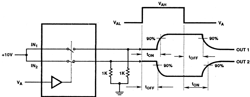
FIGURE 11. ON/OFF SWITCH TIME vs LOGIC LEVEL
