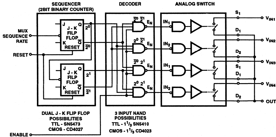
FIGURE 11. 4 - CHANNEL SEQUENCING MUX
