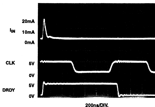
FIGURE 18. TYPICAL ANALOG INPUT CURRENT
