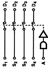
FIGURE 4. 4PST
