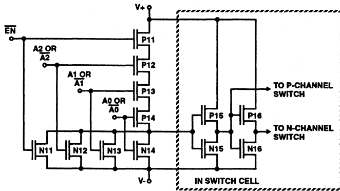
ADDRESS DECODER
