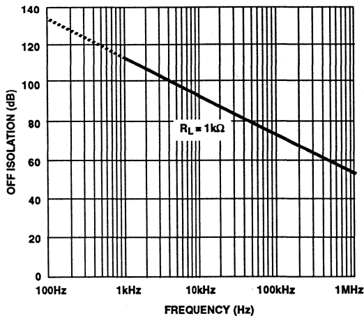
FIGURE 8. OFF ISOLATION vs FREQUENCY
