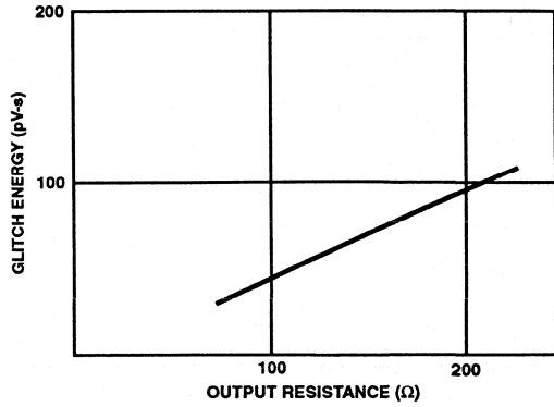
FIGURE 5. OUTPUT RESISTANCE vs GLITCH ENERGY
