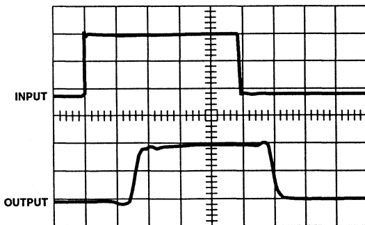
Top: TTL Input (1V/Div.) V_{AH} = 5V , V_{AL} = 0V Bottom: Output (2V/Div.) Horizontal: 200ns/Div.
