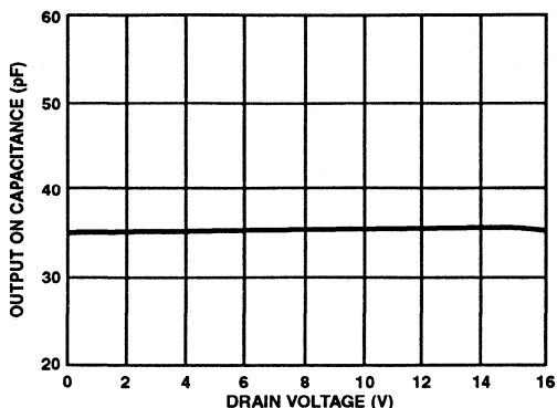
FIGURE 8. OUTPUT ON CAPACITANCE vs DRAIN VOLTAGE
