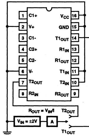
FIGURE 9. POWER-OFF SOURCE RESISTANCE CONFIGURATION
