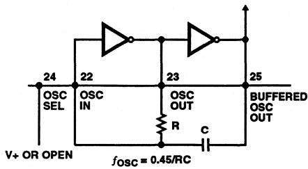
FIGURE 10. RC OSCILLATOR
