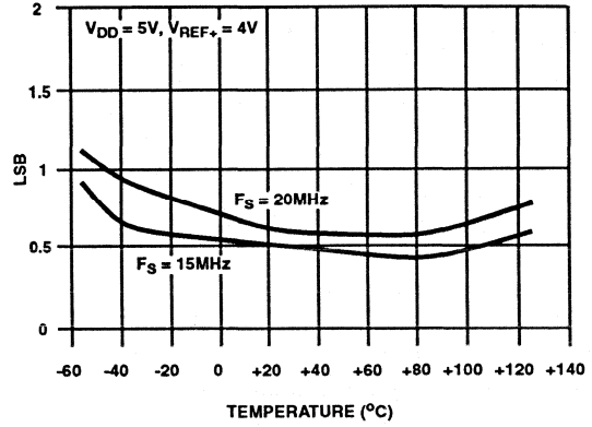
FIGURE 10. FULL SCALE ERROR vs. TEMPERATURE
