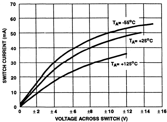
FIGURE 6A. ON CHANNEL CURRENT vs VOLTAGE
