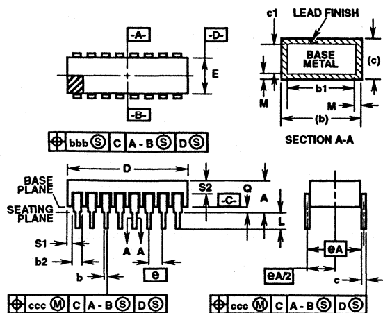
D40.6 MIL-STD-1835 CDIP2-T40 (D-5, CONFIGURATION C) 40 LEAD METAL SEAL DUAL-IN-LINE CERAMIC PACKAGE
