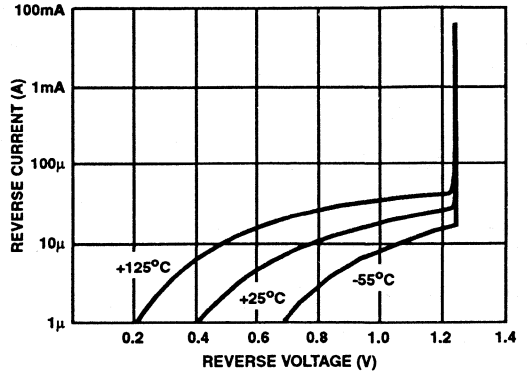
FIGURE 2. REVERSE VOLTAGE AS A FUNCTION OF CURRENT
