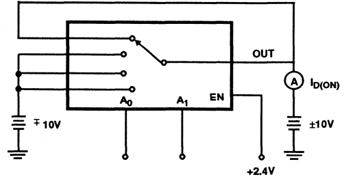
FIGURE 2D. I_{D(ON)} TEST CIRCUIT
