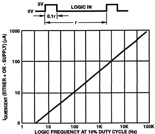
FIGURE 5. POWER SUPPLY QUIESCENT CURRENT vs LOGIC FREQUENCY RATE
