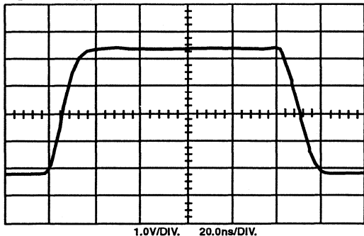
FIGURE 5. OUTPUT WAVEFORM ( C_L = 40\text{pF} )
