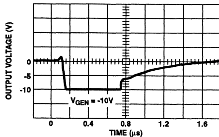
9G. V_{OUT} vs TIME
