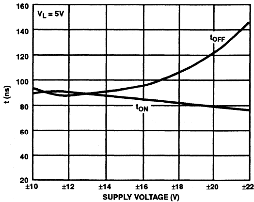
FIGURE 11. SWITCHING TIME vs POWER SUPPLY VOLTAGE (DG445)
