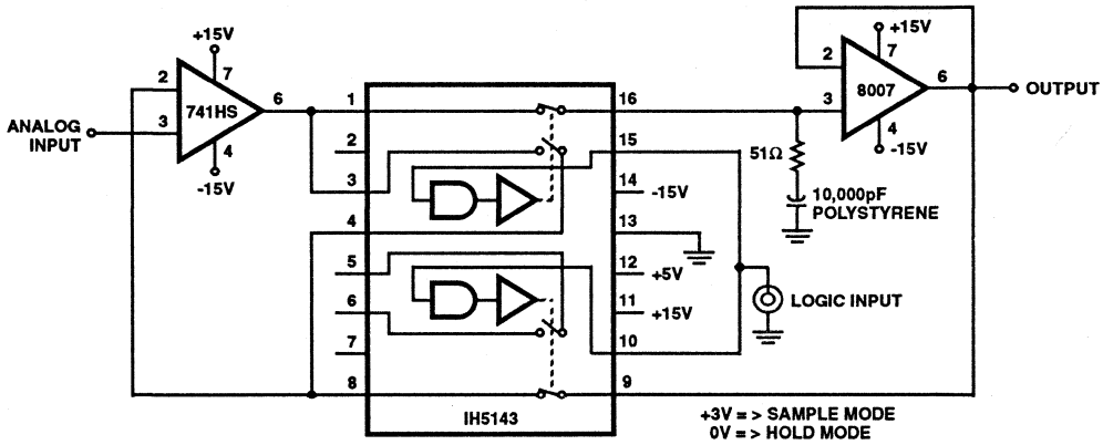
FIGURE 19. IMPROVED SAMPLE AND HOLD USING IH5143
