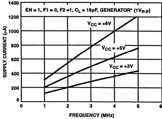
FIGURE 12. SUPPLY CURRENT vs FREQUENCY
