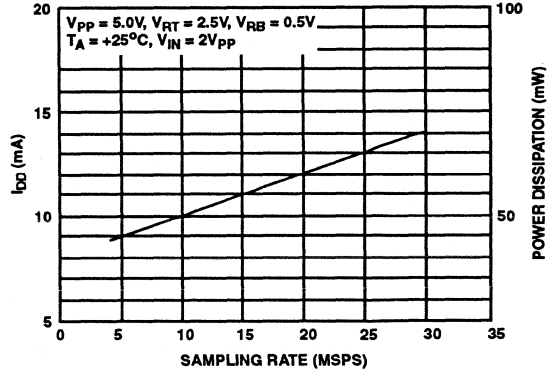
FIGURE 4. SUPPLY CURRENT AND POWER vs SAMPLING RATE
