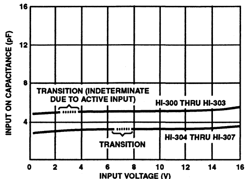
FIGURE 9. DIGITAL INPUT CAPACITANCE vs INPUT VOLTAGE
