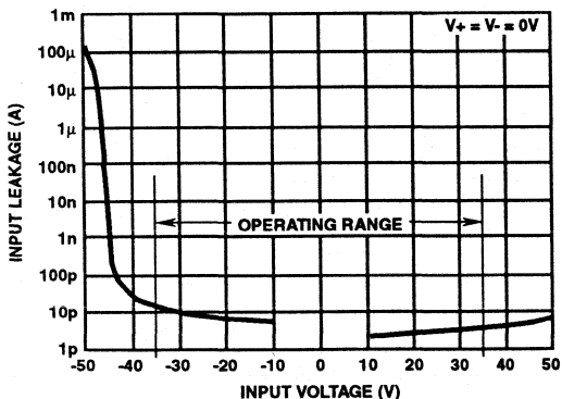
FIGURE 1. INPUT LEAKAGE vs INPUT VOLTAGE
