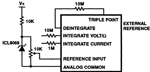
FIGURE 13. EXTERNAL VOLTAGE REFERENCE CONNECTION TO ICL7139 AND ICL7149
