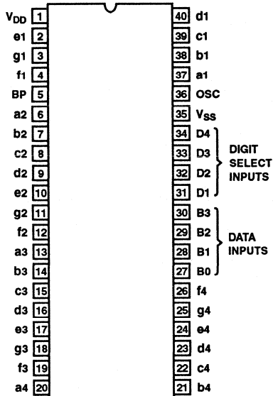
ICM7211, ICM7211A (PDIP) TOP VIEW
