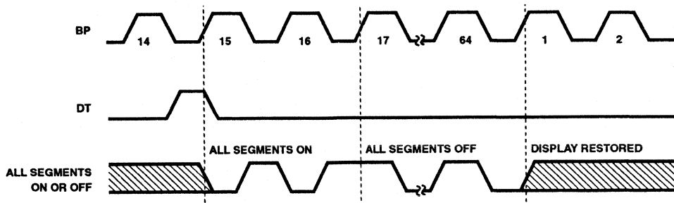
FIGURE 6. DISPLAY TESTING
