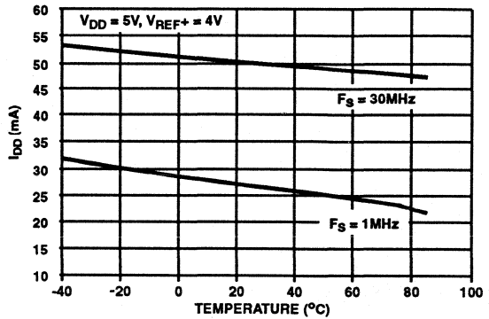
FIGURE 10. SUPPLY CURRENT vs TEMPERATURE
