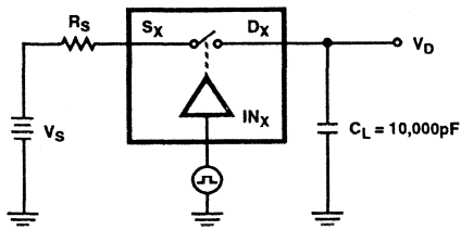
FIGURE 1. CHARGE INJECTION TEST CIRCUIT
