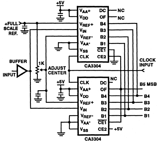
FIGURE 13. TYPICAL CA3304 5-BIT CONFIGURATION
