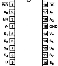
DG528 (PDIP, SOIC) TOP VIEW
