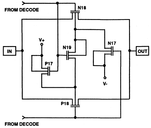
MULTIPLEX SWITCH
