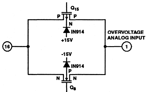
FIGURE 12. FAULT CONDITION WITH PROTECTION DIODES
