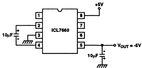
FIGURE 12. GENERATING A NEGATIVE SUPPLY FROM +5V
