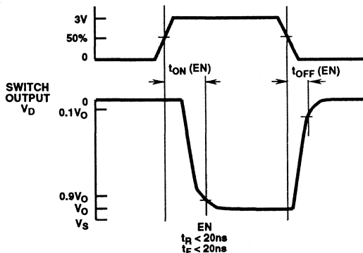
FIGURE 5C. ENABLE t_{ON} AND t_{OFF} SWITCHING TIME WAVEFORMS
