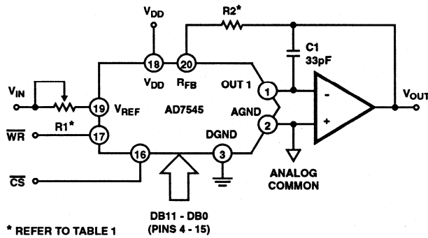
FIGURE 5. UNIPOLAR BINARY OPERATION
