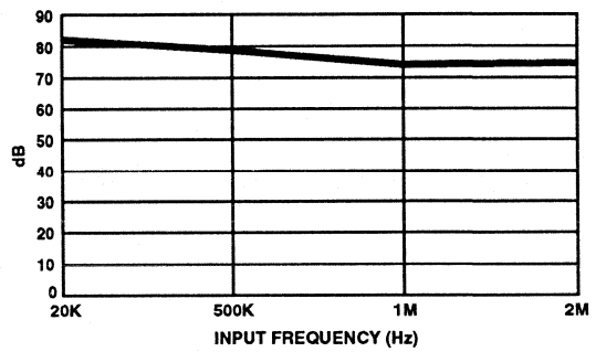
FIGURE 5. TYPICAL THD vs INPUT FREQUENCY
