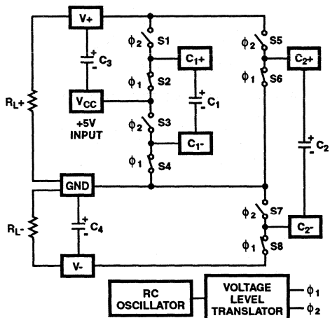
FIGURE 3. DUAL CHARGE PUMP
