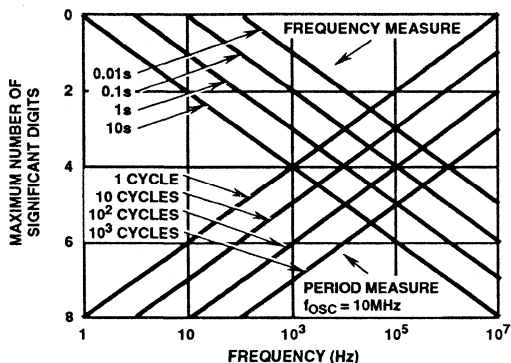
FIGURE 14. MAXIMUM ACCURACY OF FREQUENCY AND PERIOD MEASUREMENTS DUE TO LIMITATIONS OF QUANTIZATION ERRORS
