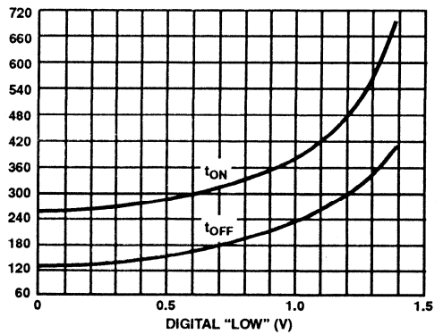
FIGURE 13. SWITCHING TIMES FOR NEGATIVE DIGITAL TRANSITION
