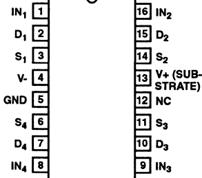
DG201A, DG202 (CDIP, PDIP, SOIC) TOP VIEW
