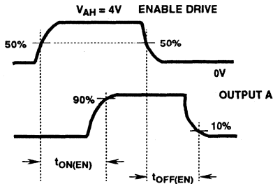
FIGURE 6A. t_{ON(EN)} , t_{OFF(EN)} MEASUREMENT
