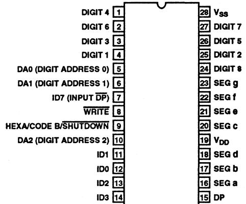
ICM7228D (CDIP, PCIP SOIC) COMMON CATHODE TOP VIEW
