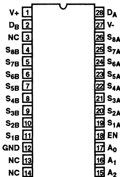
DG507A (PDIP, CDIP, SOIC) TOP VIEW
