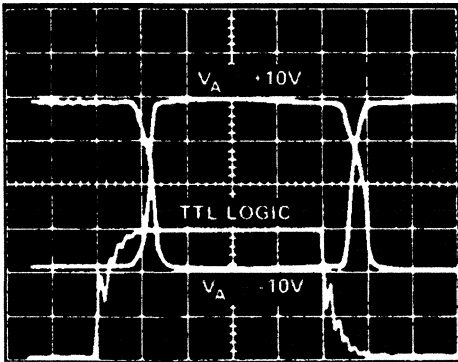
FIGURE 17. +25°C TTL OPEN COLLECTOR LOGIC DRIVE (Corresponds to Figure 14)
