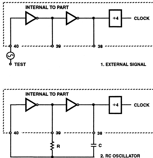
FIGURE 7. CLOCK CIRCUITS
