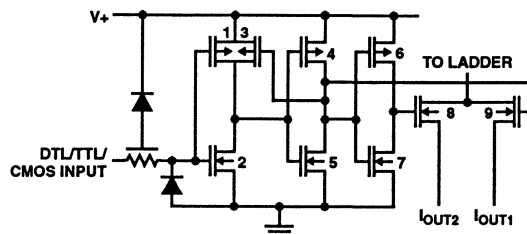
FIGURE 1. CMOS SWITCH
