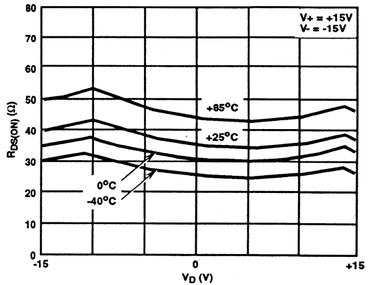
FIGURE 4. R_{DS(ON)} vs V_D AND TEMPERATURE
