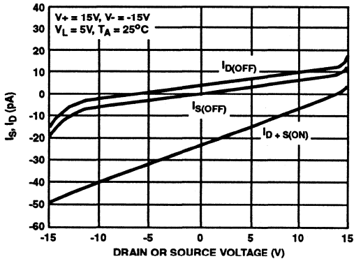
FIGURE 3. LEAKAGE CURRENT vs ANALOG VOLTAGE
