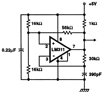
FIGURE 11. LM311 CLOCK SOURCE
