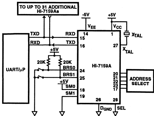
FIGURE 4C. SERIAL MODE 2
