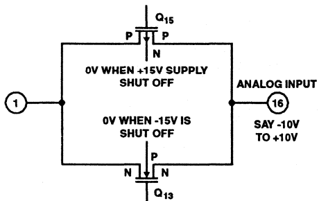
FIGURE 11. FAULT CONDITION WITHOUT PROTECTION DIODES
