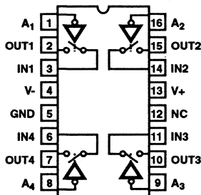
HI-201HS (CDIP, PDIP, SOIC) TOP VIEW
