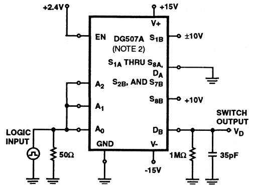
FIGURE 3B. t_{TRANSITION} SWITCHING TIME TEST CIRCUIT
