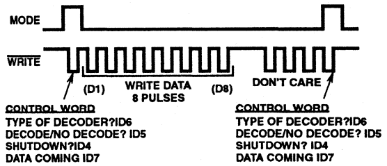
FIGURE 2. ICM7228A/B SEQUENTIAL 8 DIGIT RAM UPDATE
