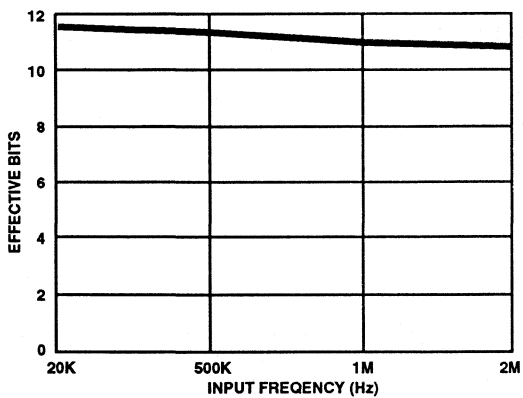
FIGURE 8. TYPICAL EFFECTIVE BITS vs INPUT FREQUENCY
