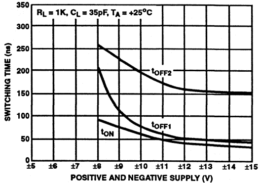
FIGURE 11. SWITCHING TIME vs POSITIVE AND NEGATIVE SUPPLY VOLTAGE
