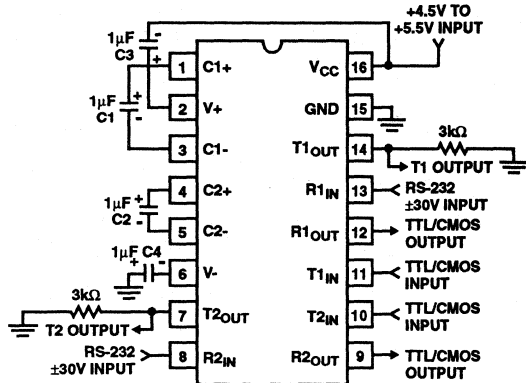
FIGURE 8. GENERAL TEST CIRCUIT
