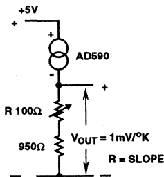
FIGURE 2. SLOPE TRIMMING
