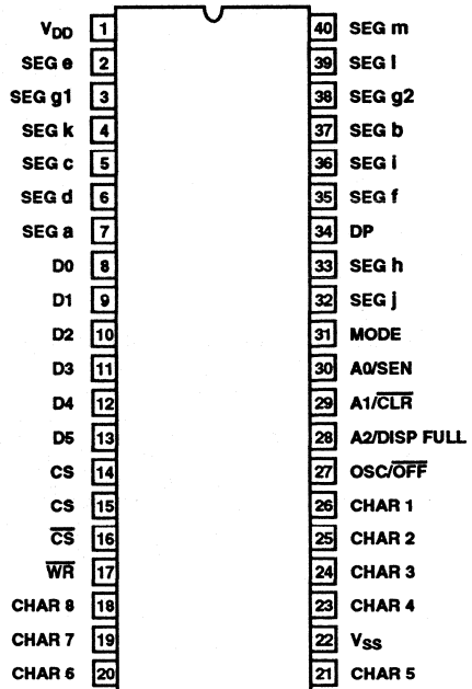
ICM7243B (14-SEGMENT CHARACTER) (PDIP) TOP VIEW
