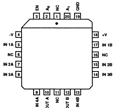
HI4P539 (PLCC) TOP VIEW
