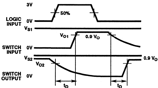
FIGURE 8. BREAK-BEFORE-MAKE
