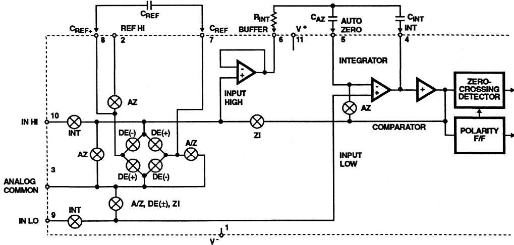
FIGURE 3. ANALOG SECTION OF ICL7135
