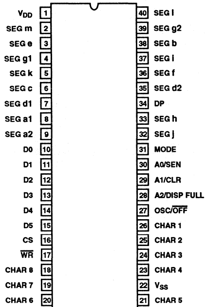
ICM7243A (16-SEGMENT CHARACTER) (PDIP) TOP VIEW
