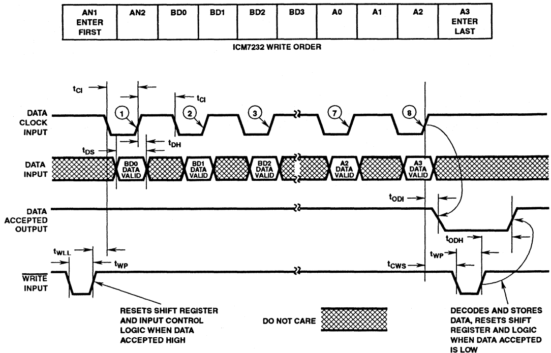
FIGURE 3. ICM7232 INPUT TIMING DIAGRAM, LEAVING BOTH ANNUNCIATORS OFF
