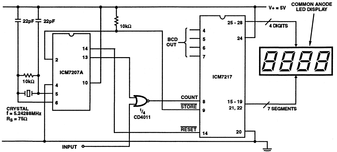
FIGURE 23. PRECISION FREQUENCY COUNTER (MHZ MAXIMUM)
