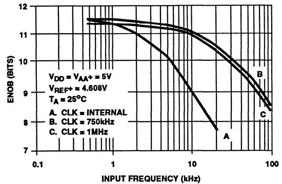
FIGURE 15. EFFECTIVE BITS vs INPUT FREQUENCY
