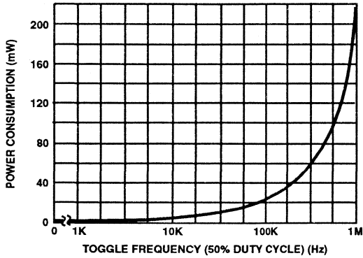
FIGURE 10. POWER CONSUMPTION vs FREQUENCY
