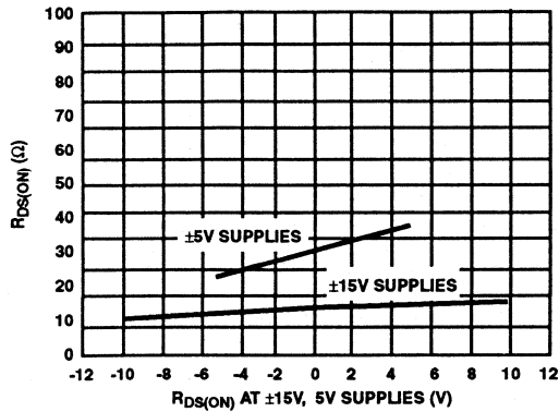
FIGURE 1. R_{DS(ON)} vs ANALOG INPUT VOLTAGE
