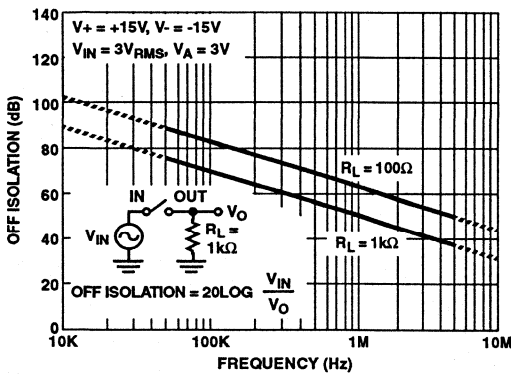
FIGURE 18. OFF ISOLATION vs FREQUENCY
