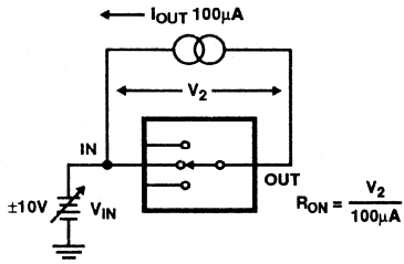
FIGURE 1. ON RESISTANCE vs INPUT SIGNAL LEVEL
