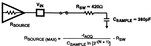
FIGURE 14. ANALOG INPUT MODEL IN TRACK MODE
