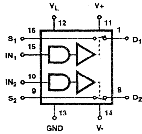
DIP (JE, PE) DUAL SPST IH5141
