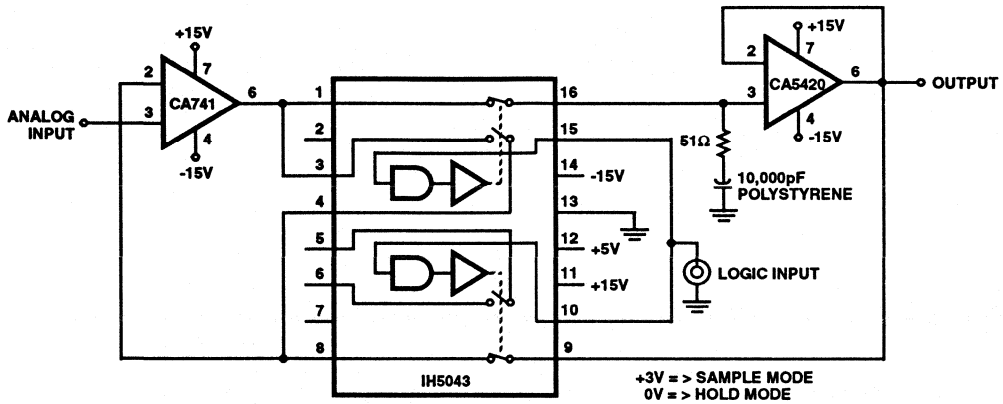
FIGURE 10. IMPROVED SAMPLE AND HOLD
