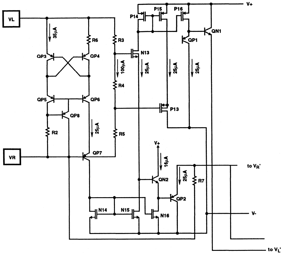
FIGURE 14. TTL/CMOS REFERENCE CIRCUIT (Note 1)
