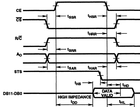
FIGURE 5. READ CYCLE TIMING
