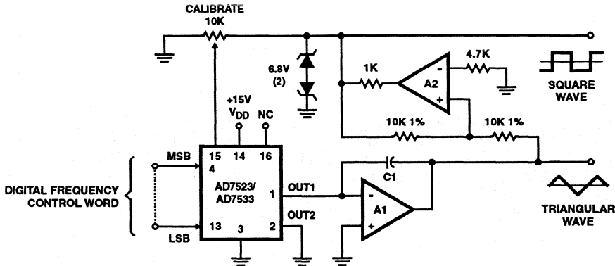
FIGURE 5. PROGRAMMABLE FUNCTION GENERATOR
