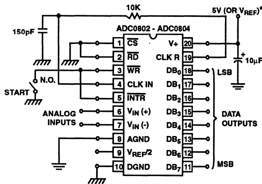
FIGURE 17. FREE-RUNNING CONNECTION
