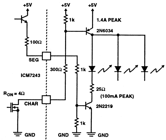
FIGURE 9B. COMMON ANODE DISPLAY
