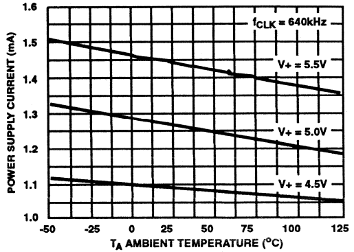
FIGURE 9. POWER SUPPLY CURRENT vs TEMPERATURE
