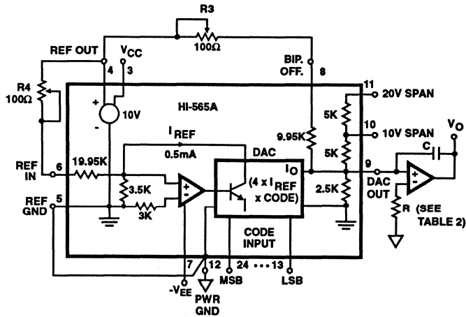
FIGURE 2. BIPOLAR VOLTAGE OUTPUT
