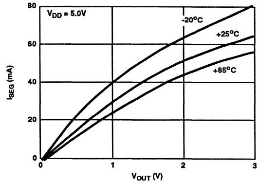
FIGURE 7. ICM7226A TYPICAL I_{SEG} vs V_{OUT}
