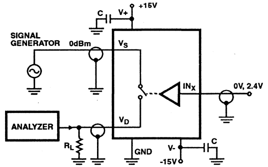
FIGURE 11. OFF ISOLATION
