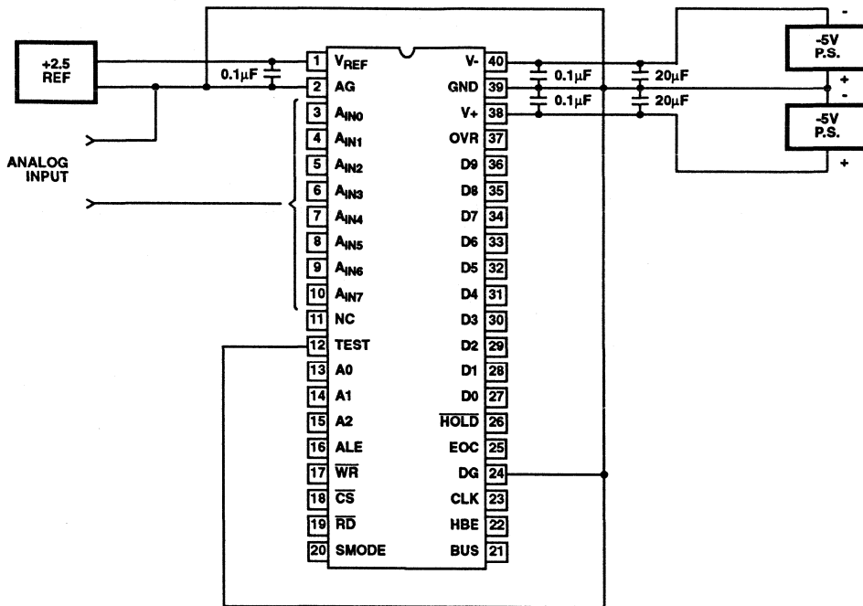
FIGURE 3. GROUND AND POWER SUPPLY DECOUPLING
