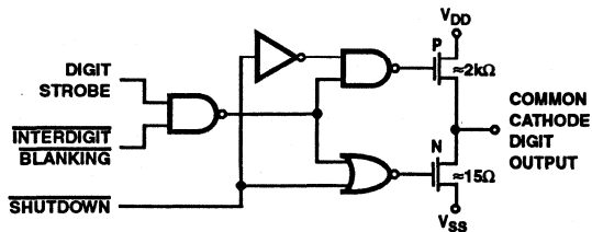
13A. DIGIT DRIVER
