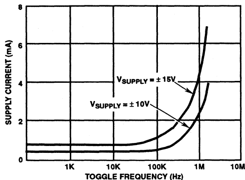
FIGURE 5A. SUPPLY CURRENT vs TOGGLE FREQUENCY
