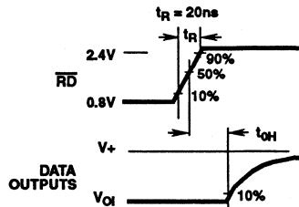
FIGURE 1D. t_{OH} , C_L = 10pF
