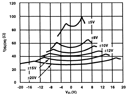
FIGURE 15. r_{DS(ON)} vs V_D AND SUPPLY
