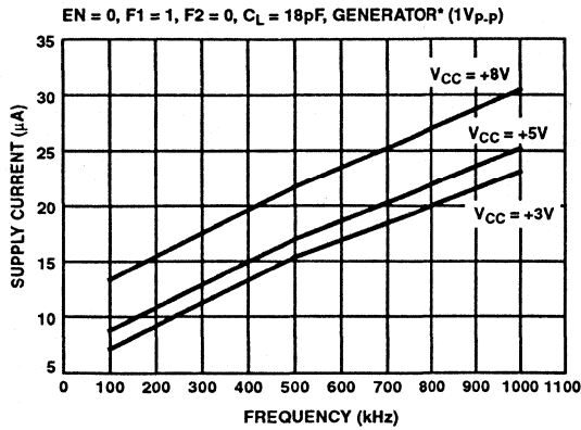
FIGURE 17. DISABLE SUPPLY CURRENT vs FREQUENCY
