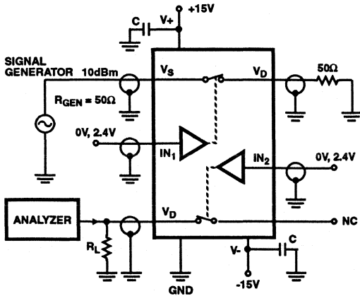
FIGURE 20. CROSSTALK
