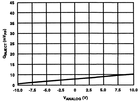
FIGURE 6. CHARGE INJECTION vs V_{ANALOG} (SEE FIGURE 8) C_L = 10,000pF
