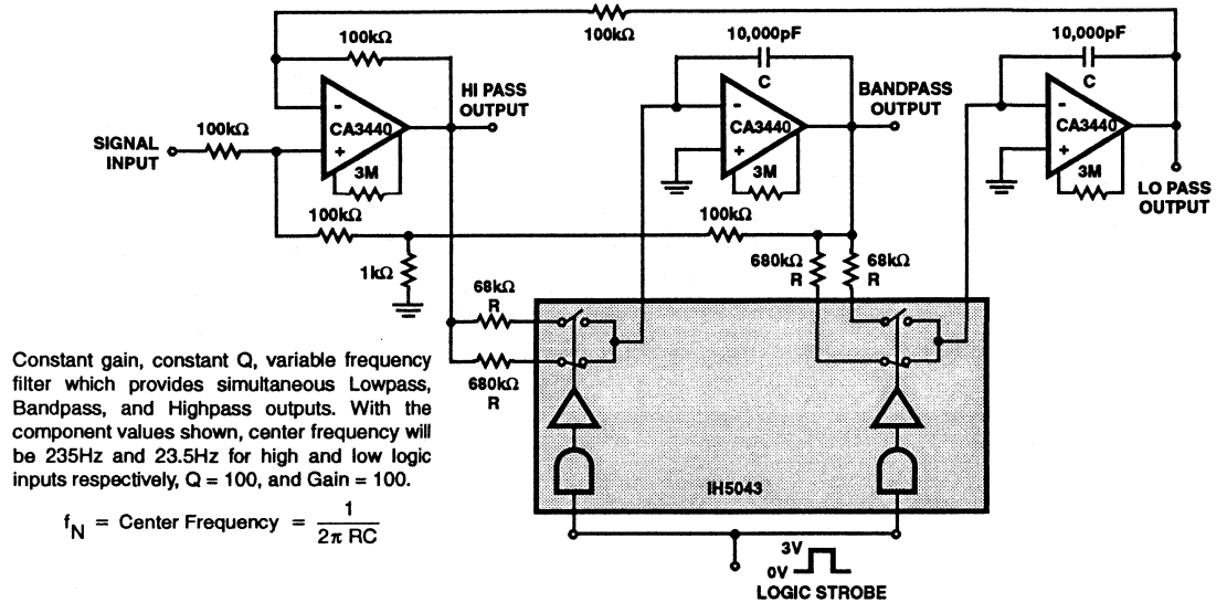
FIGURE 12. DIGITALLY TUNED LOW POWER ACTIVE FILTER
