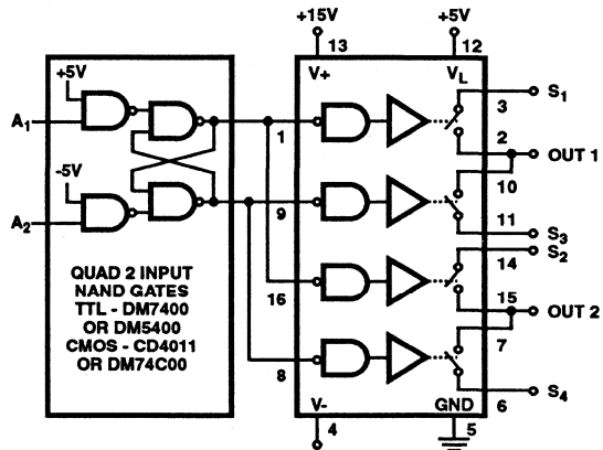
FIGURE 12. A LATCHING DPDT
