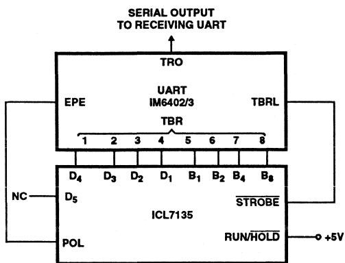
FIGURE 13. ICL7135 TO UART INTERFACE
