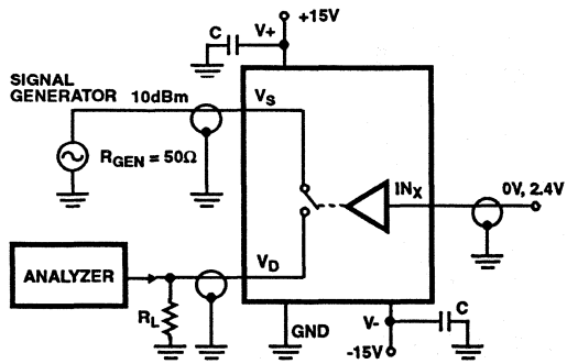
FIGURE 21. OFF ISOLATION
