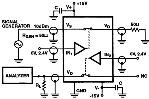
FIGURE 20. CROSTALK
