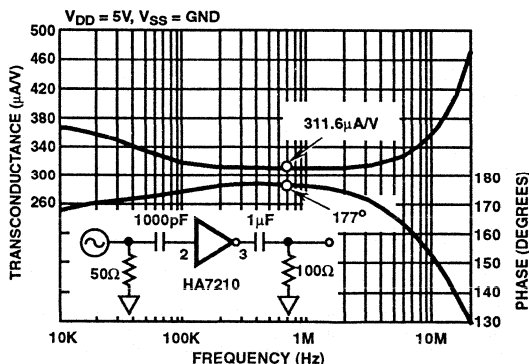
FIGURE 36. TRANSCONDUCTANCE vs FREQUENCY F1 = 0, F2 = 1
