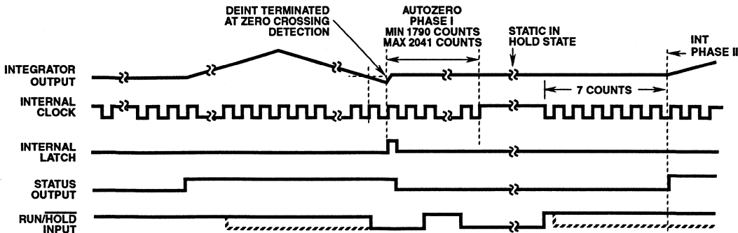
FIGURE 5. RUN/HOLD OPERATION
