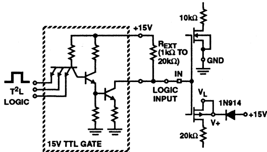
FIGURE 13. INTERFACING WITH TTL OPEN COLLECTOR LOGIC (TYP EXAMPLE FOR +15V CASE SHOWN)
