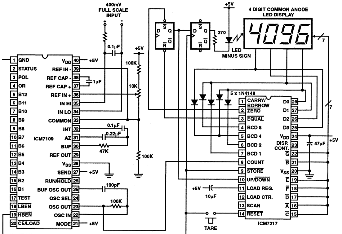
FIGURE 24. AUTO-TARE SYSTEM FOR A/D CONVERTER
