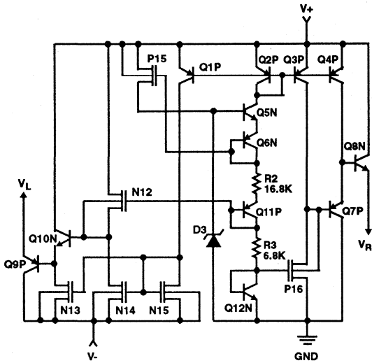
TTL REFERENCE CIRCUIT
