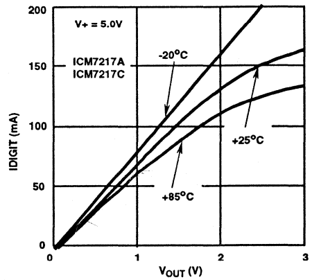
FIGURE 7. TYPICAL IDIGIT vs V_{OUT}
