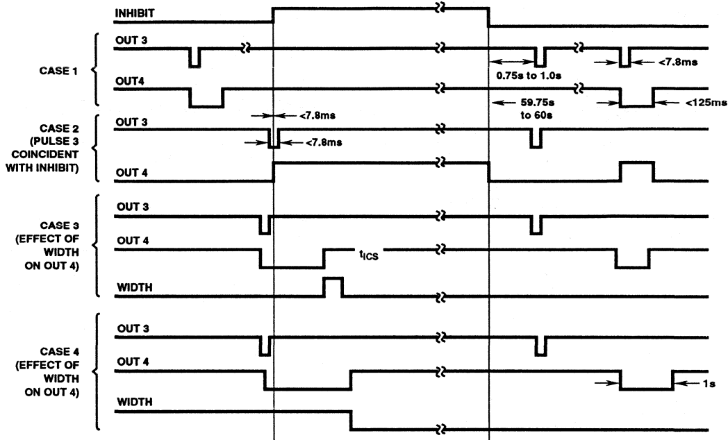
FIGURE 2. EFFECT OF THE INHIBIT (TEST CONNECTED TO V_{SS} OR LEFT OPEN)
