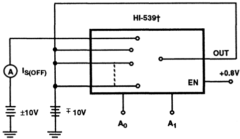
FIGURE 2C. I_{S(OFF)} TEST CIRCUIT (NOTE 1)
