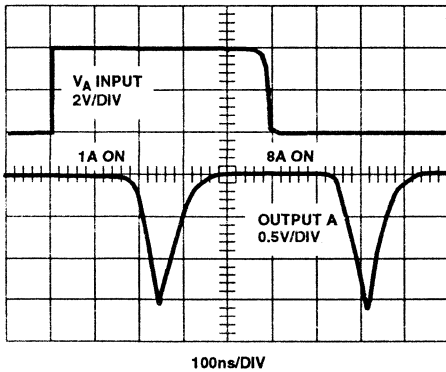
FIGURE 8C. BREAK-BEFORE-MAKE DELAY WAVEFORMS
