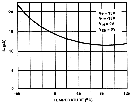
FIGURE 13. POSITIVE SUPPLY CURRENT vs TEMPERATURE (DG408)
