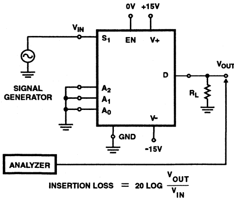
FIGURE 31. INSERTION LOSS
