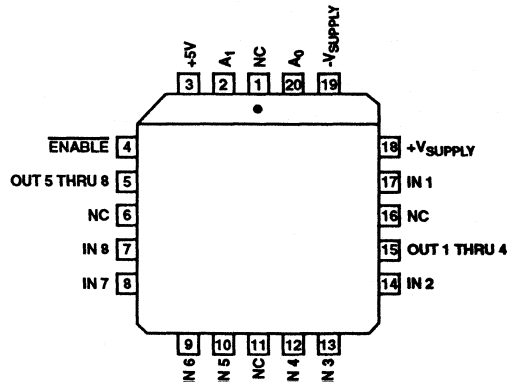
HI-1828A (CLCC, PLCC) TOP VIEW
