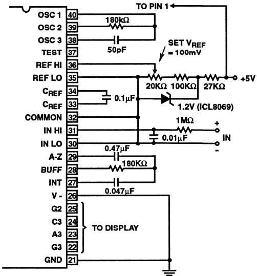
FIGURE 16. ICL7137 OPERATED FROM SINGLE +5V
