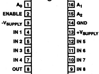
HI-508 (PDIP, CDIP, SOIC) TOP VIEW
