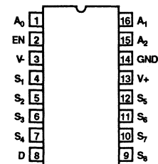
DG508A (PDIP, CDIP, SOIC) TOP VIEW
