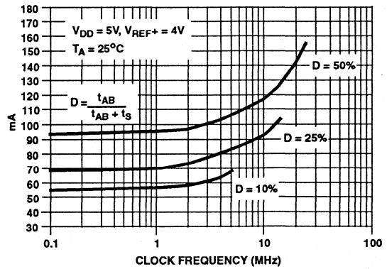
FIGURE 14. SUPPLY CURRENT vs. CLOCK & DUTY CYCLE
