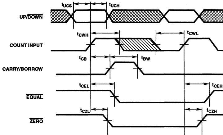
FIGURE 2. COUNT AND OUTPUTS TIMING
