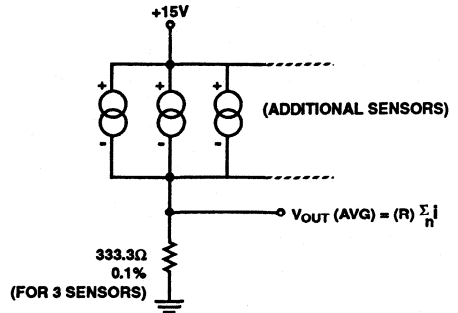
FIGURE 8. AVERAGE TEMPERATURE SENSING SCHEME
