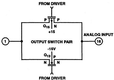
FIGURE 10. SWITCH WITHOUT PROTECTION DIODES
