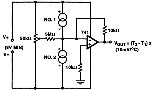
FIGURE 15. DIFFERENTIAL THERMOMETER
