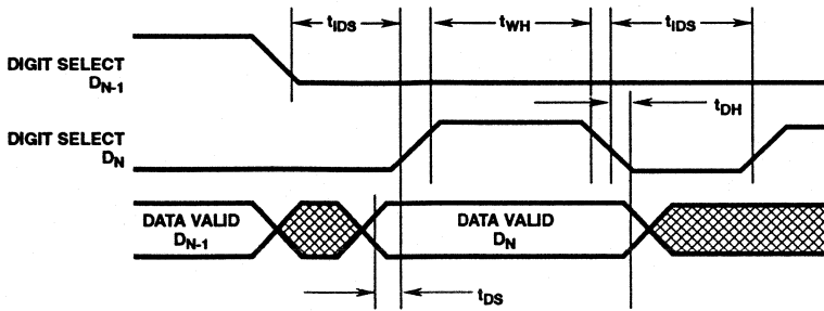
FIGURE 1. MULTIPLEXED INPUT
