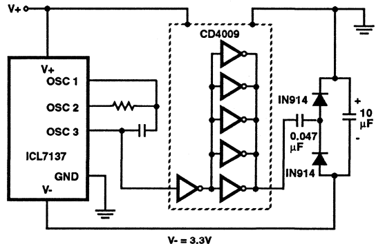
FIGURE 10. GENERATING NEGATIVE SUPPLY FROM +5V
