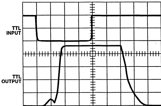
FIGURE 7. TTL INPUT
