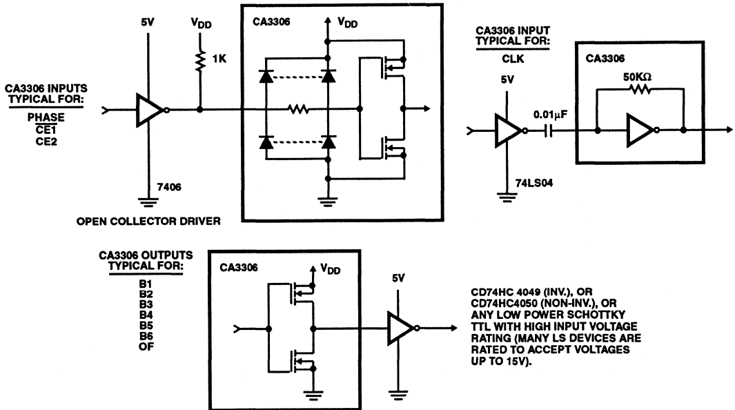
FIGURE 20. 5V LOGIC INTERFACE CIRCUIT FOR V_{DD} > 5.5V
