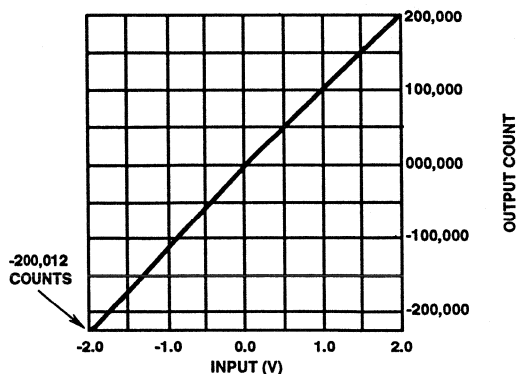
FIGURE 9. TYPICAL HI-7159A TRANSFER CHARACTERISTIC
