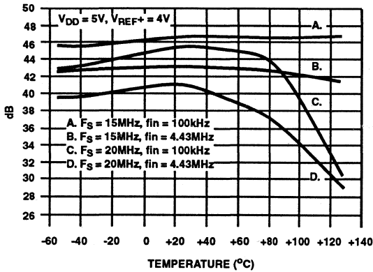
FIGURE 5. SNR vs TEMPERATURE
