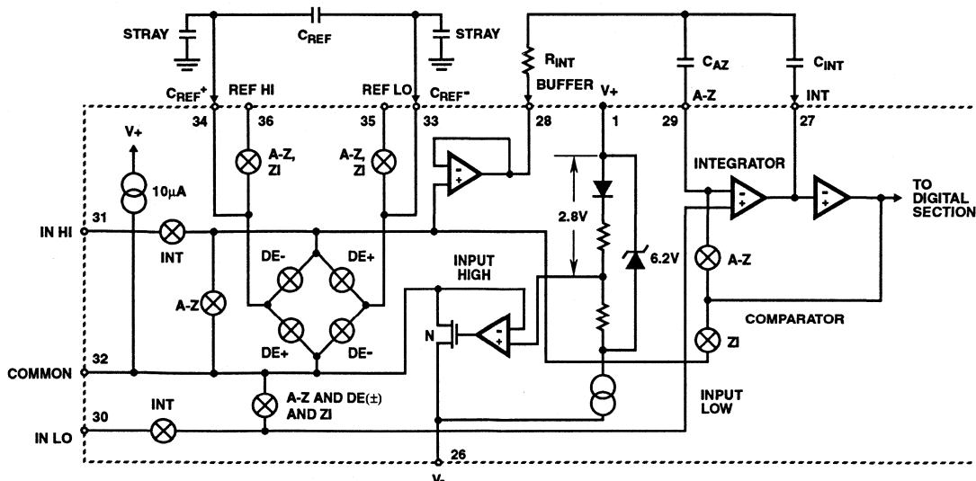
FIGURE 3. ANALOG SECTION OF ICL7136 AND ICL7137
