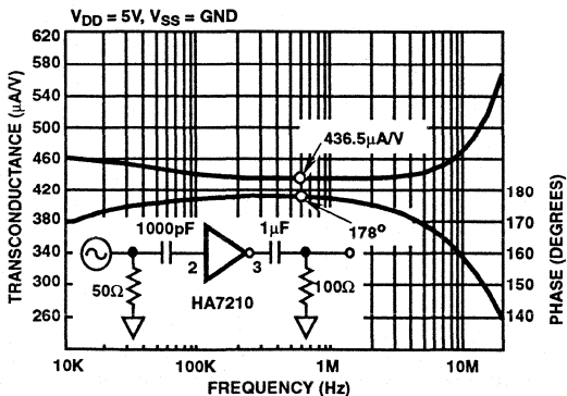
FIGURE 35. TRANSCONDUCTANCE vs FREQUENCY F1 = 0, F2 = 0
