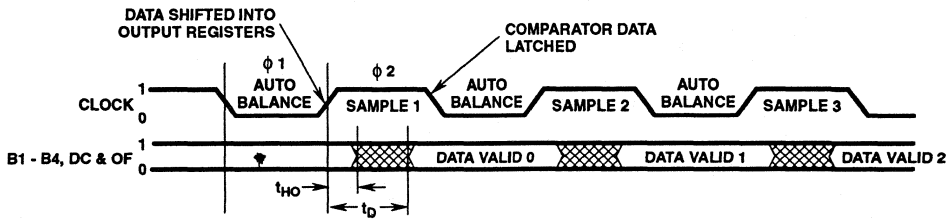
FIGURE 1. TIMING DIAGRAM
