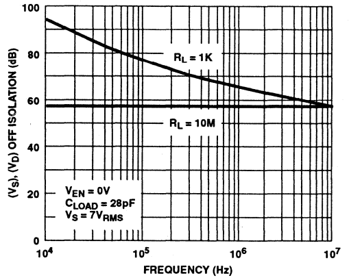
FIGURE 4. OFF ISOLATION vs FREQUENCY
