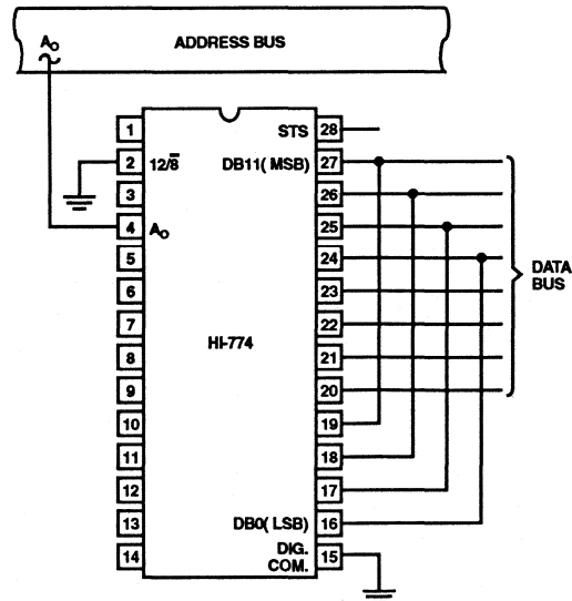
FIGURE 6. INTERFACE TO AN 8 BIT DATA BUS
