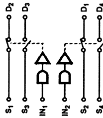
FIGURE 6. DUAL SPDT
