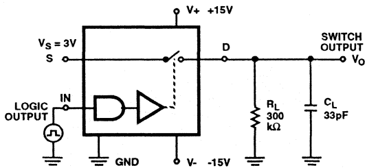
FIGURE 3. t_{ON} and t_{OFF} TEST CIRCUIT
