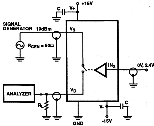
FIGURE 21. OFF ISOLATION
