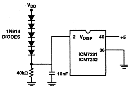
FIGURE 11A. STRING OF DIODES
