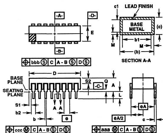
D42.6 42 LEAD METAL SEAL DUAL-IN-LINE CERAMIC PACKAGE
