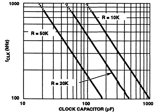
FIGURE 5. f_{\text{CLK}} vs CLOCK CAPACITOR
