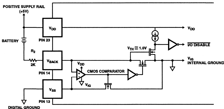
FIGURE 5. SIMPLIFIED ICM7170 BATTERY BACKUP CIRCUIT
