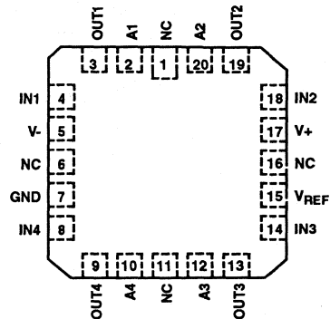
HI-201 (20 PIN PLCC, CLCC) TOP VIEW
