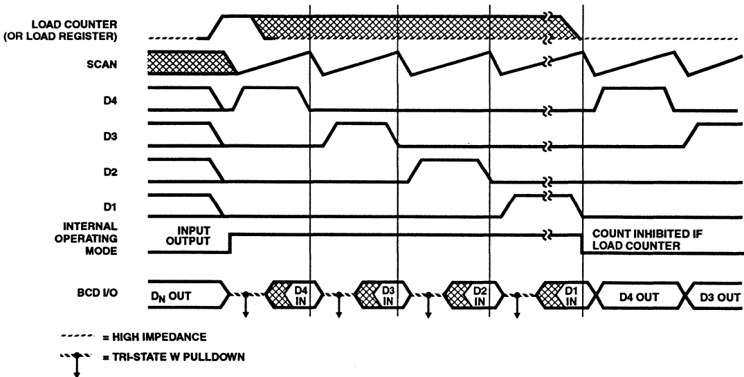
FIGURE 3. BCD I/O AND LOADING TIMING
