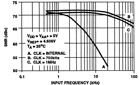
FIGURE 17. SIGNAL NOISE RATIO vs INPUT FREQUENCY
