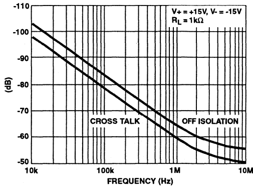
FIGURE 11. OFF ISOLATION AND CROSS TALK vs FREQUENCY
