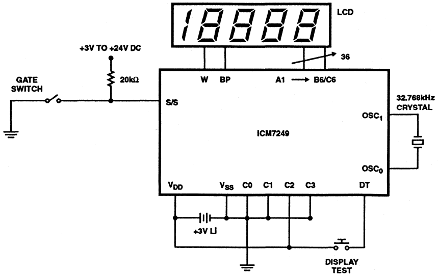
FIGURE 9. ATTENDANCE COUNTER
