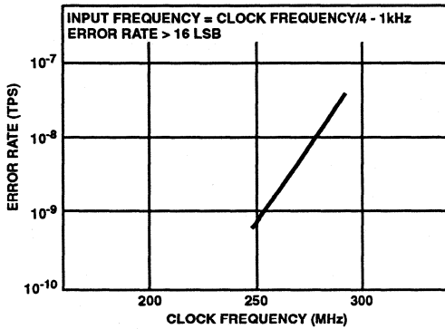
FIGURE 14. ERROR RATE vs CONVERSION RATE
