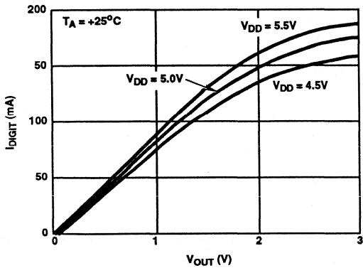
FIGURE 2. ICM7226B TYPICAL I_{DIGIT} vs V_{OUT}
