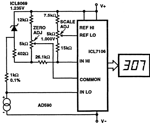
FIGURE 13. BASIC DIGITAL THERMOMETER, KELVIN SCALE WITH ZERO ADJUST
