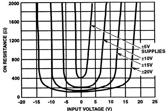
FIGURE 4. R_{DS(ON)} vs INPUT VOLTAGE
