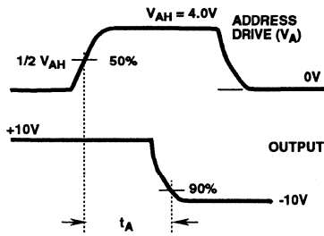
FIGURE 7A. ACCESS TIME MEASUREMENT
