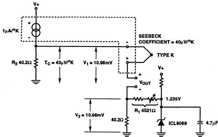
FIGURE 16. COLD JUNCTION COMPENSATION FOR TYPE K THERMOCOUPLE
