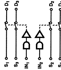
FIGURE 8. DUAL DPST
