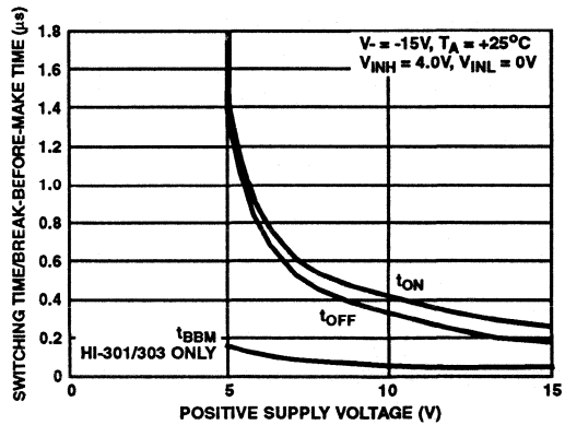
FIGURE 15. SWITCHING TIME AND BREAK-BEFORE-MAKE TIME vs POSITIVE SUPPLY VOLTAGE, HI-300 THRU HI-303
