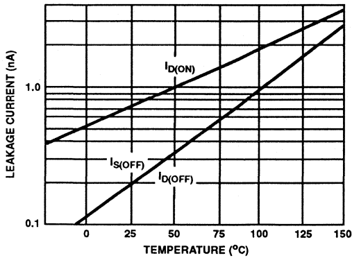
FIGURE 3. LEAKAGE CURRENT vs TEMPERATURE
