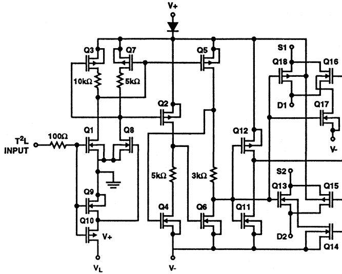
TYPICAL DRIVER/GATE - IH5142
