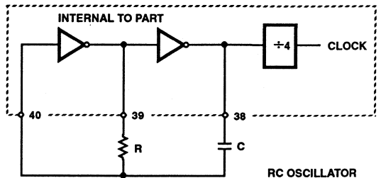
FIGURE 9. CLOCK CIRCUITS
