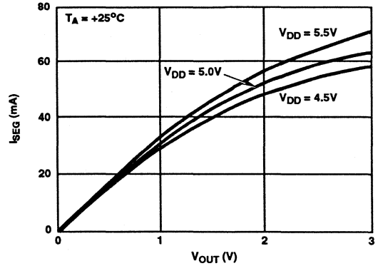
FIGURE 5. ICM7226A TYPICAL I_{SEG} vs V_{OUT}
