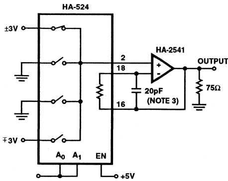
TEST CIRCUIT 5. SETTLING TIME, ACCESS TIME, BREAK-BEFORE-MAKE DELAY (NOTE 2)
