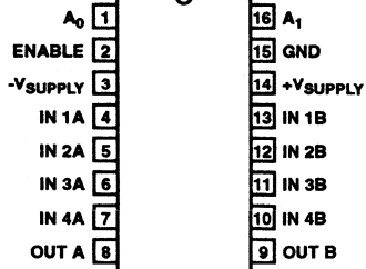
HI-509 (PDIP, CDIP, SOIC) TOP VIEW
