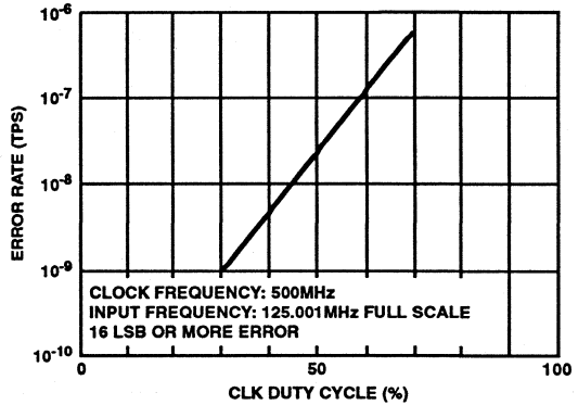
FIGURE 11. ERROR RATE vs CLOCK DUTY CYCLE CHARACTERISTICS
