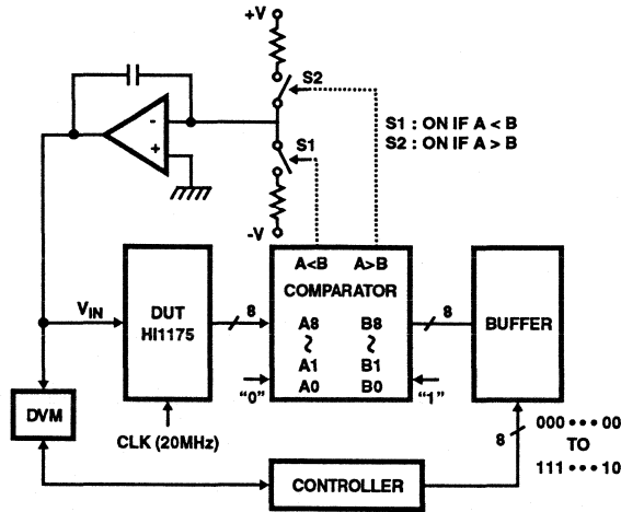
FIGURE 6. INTEGRAL AND DIFFERENTIAL NON-LINEARITY ERROR AND OFFSET VOLTAGE TEST CIRCUIT
