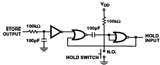
FIGURE 25. CIRCUIT FOR REDUCING TIME BETWEEN MEASUREMENTS
