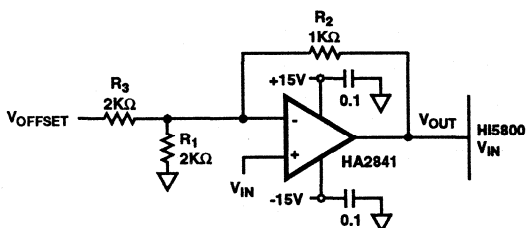
FIGURE 4. NON-INVERTING BUFFER
