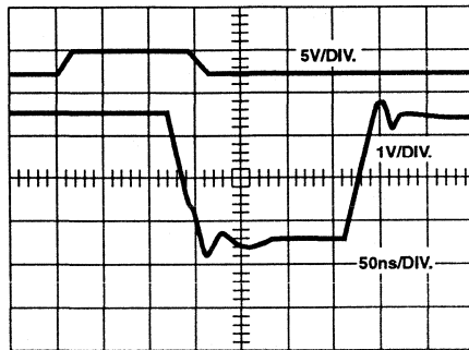
FIGURE 5. ACCESS TIME
