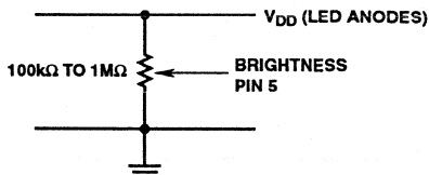
FIGURE 9. BRIGHTNESS CONTROL
