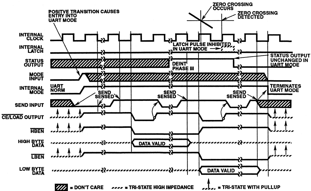
FIGURE 9. HANDSHAKE TRIGGERED BY MODE
