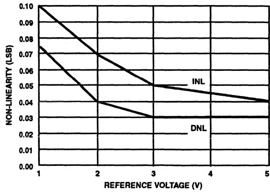
FIGURE 7. NON-LINEARITY vs REFERENCE VOLTAGE
