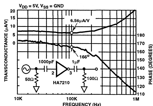
FIGURE 38. TRANSCONDUCTANCE vs FREQUENCY F1 = 1, F2 = 1
