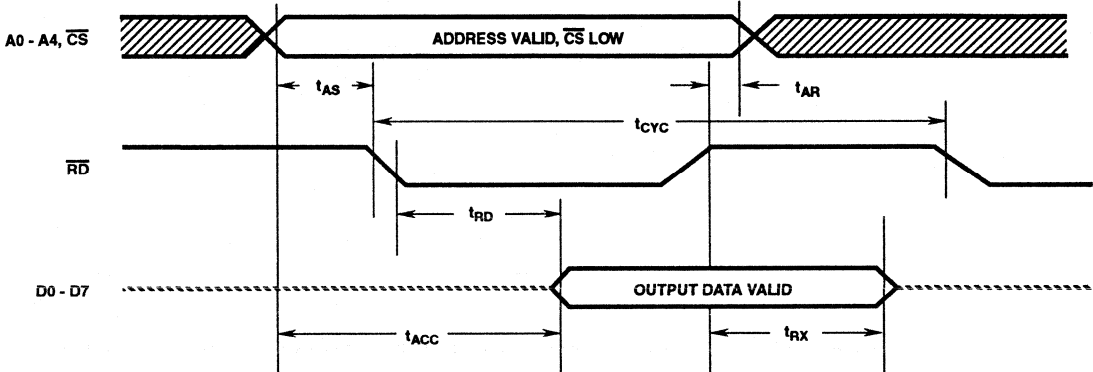
FIGURE 1. READ CYCLE TIMING FOR NON-MULTIPLEXED BUS ( ALE = V_{IH} , \overline{WR} = V_{IH} )
