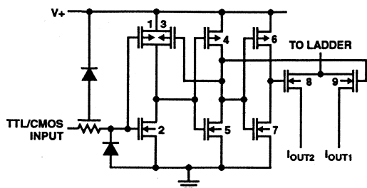
FIGURE 1. CMOS SWITCH
