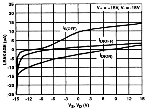
FIGURE 6. LEAKAGE CURRENT vs V_S, V_D
