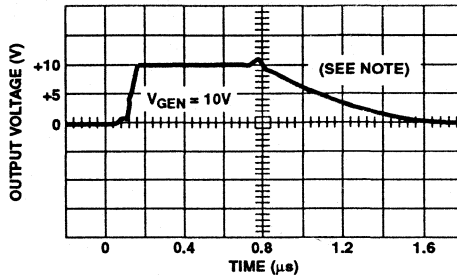
7D. V_{OUT} vs TIME
