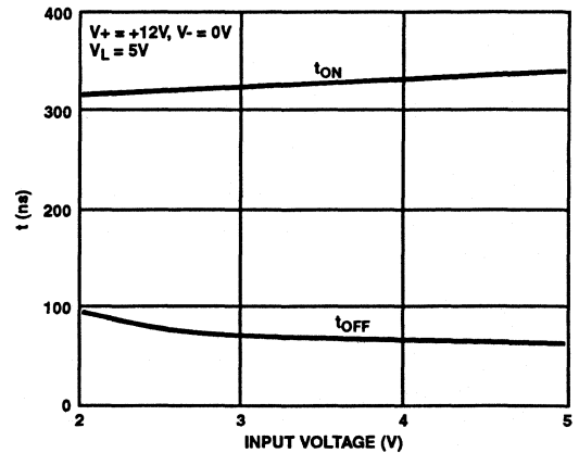
FIGURE 12. SWITCHING TIME vs INPUT VOLTAGE (DG444)
