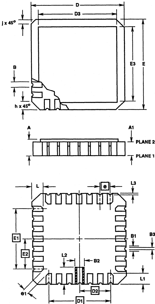
J20.A MIL-STD-1835 CQCC1-N20 (C-2) 20 PAD METAL SEAL LEADLESS CERAMIC CHIP CARRIER
