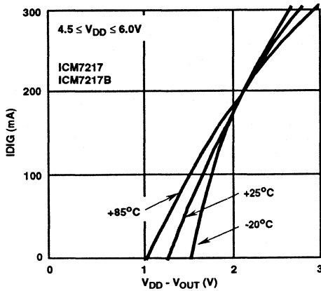
FIGURE 4. TYPICAL IDIG vs V+
