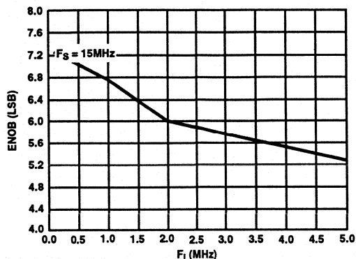
FIGURE 10. ENOB vs INPUT FREQUENCY
