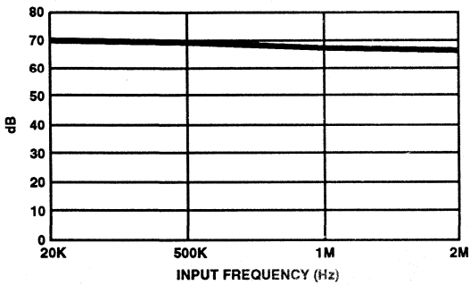
FIGURE 6. TYPICAL SND vs INPUT FREQUENCY
