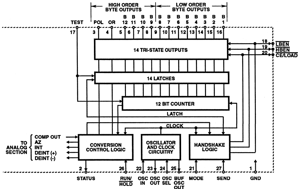
FIGURE 4. DIGITAL SECTION
