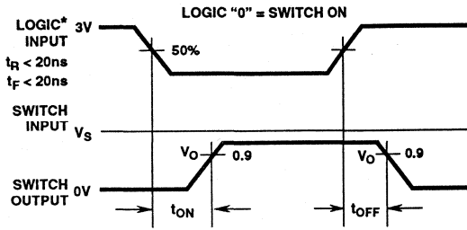
FIGURE 1. T_{ON} AND T_{OFF} SWITCHING TEST
