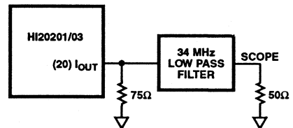
FIGURE 6. HI20201/03 GLITCH TEST CIRCUIT
