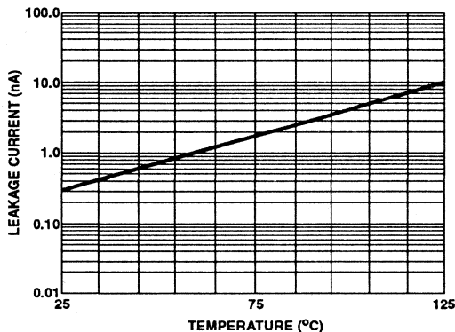
FIGURE 4. I_{S(OFF)} OR I_{D(OFF)} vs TEMPERATURE†
