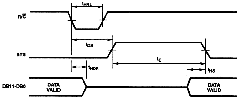
FIGURE 8. LOW PULSE FOR R/\overline{C} - OUTPUTS ENABLED AFTER CONVERSION
