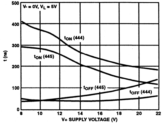
FIGURE 14. SWITCHING TIMES vs POWER SUPPLY VOLTAGE
