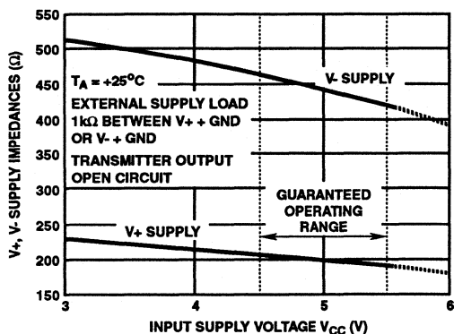
FIGURE 1. V+, V- OUTPUT IMPEDANCES vs V CC
