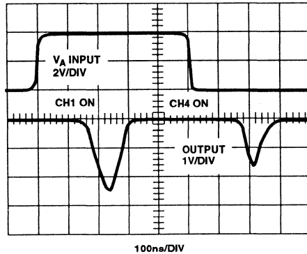
FIGURE 5C. t_{\text{OPEN}} WAVEFORMS
