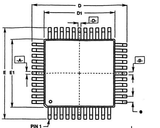
Q44.B 44 LEAD METRIC PLASTIC QUAD FLATPACK PACKAGE
