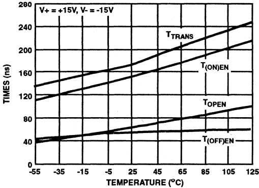
FIGURE 9. SWITCHING TIMES vs TEMPERATURE
