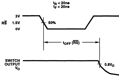
FIGURE 7A. RESET t_{OFF} SWITCHING TIME WAVEFORMS
