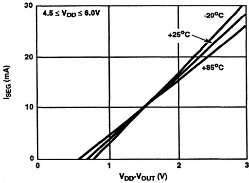
FIGURE 4. ICM7226B TYPICAL I_{SEG} vs V_{DD} - V_{OUT}
