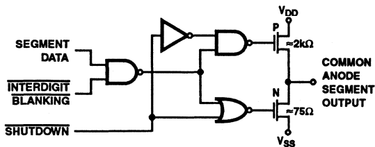
FIGURE 12B. SEGMENT DRIVER
