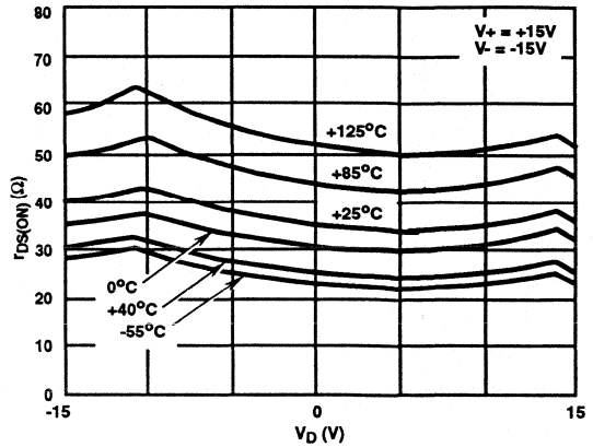
FIGURE 2. R_{DS(ON)} vs V_D AND TEMPERATURE
