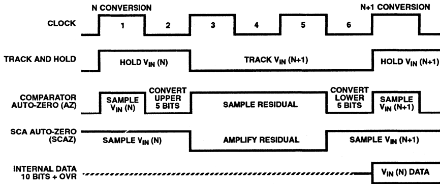
FIGURE 2. INTERNAL ADC TIMING DIAGRAM
