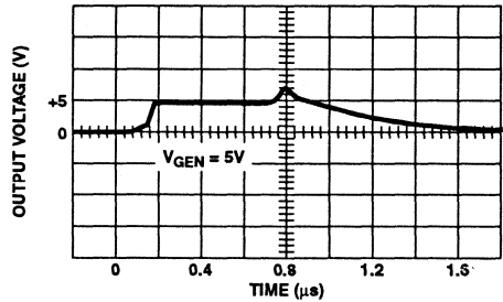
9D. V_{OUT} vs TIME
