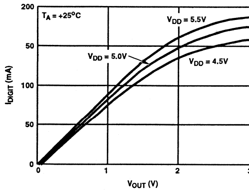
FIGURE 8. ICM7216B & ICM7216D TYPICAL I_{DIGIT} vs V_{OUT}
