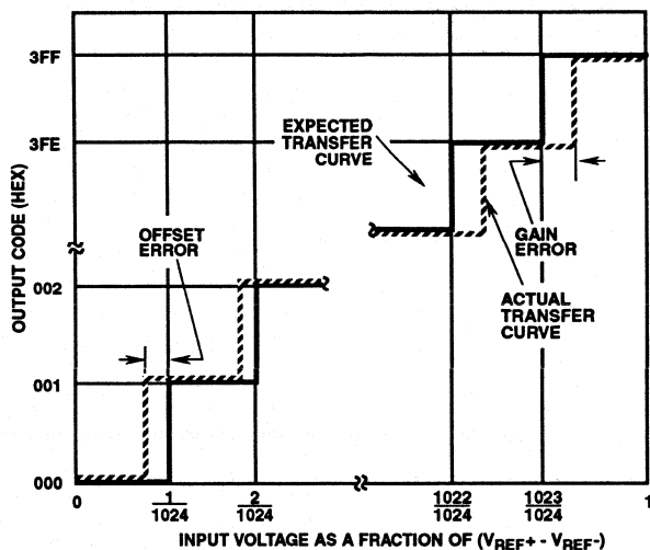
FIGURE 18. GAIN AND OFFSET ERROR
