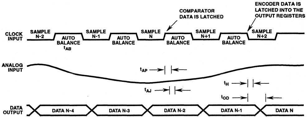
FIGURE 1. INPUT-TO-OUTPUT TIMING
