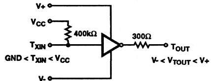
FIGURE 2. TRANSMITTER
