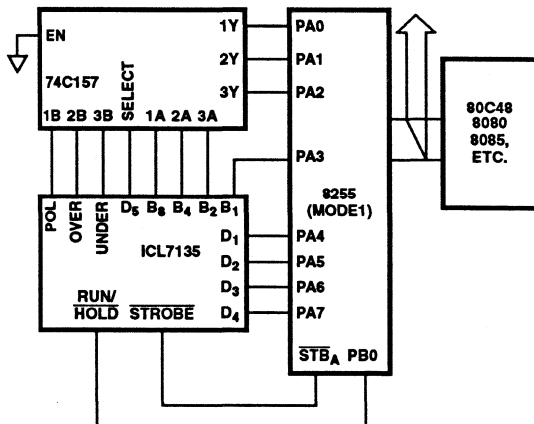
FIGURE 16. ICL7135 TO MCS-48, -80, 85 INTERFACE
