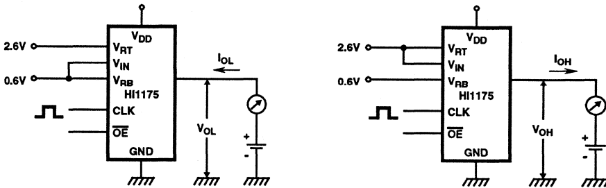
FIGURE 8. DIGITAL OUTPUT CURRENT TEST CIRCUIT
