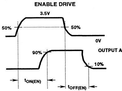
FIGURE 10B. WAVEFORMS
