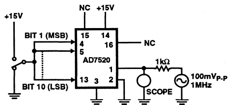
FIGURE 5. OUTPUT CAPACITANCE
