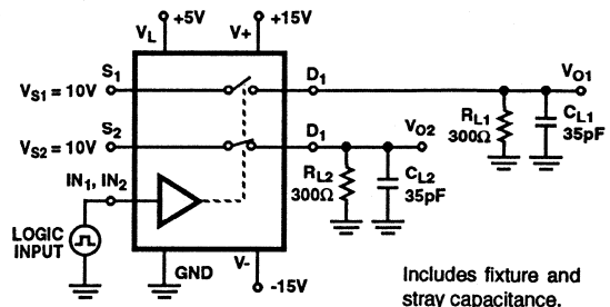
FIGURE 8. BREAK-BEFORE-MAKE
