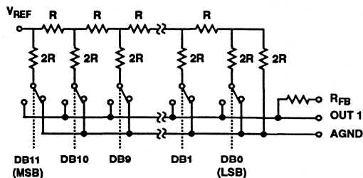
FIGURE 2. SIMPLIFIED D/A CIRCUIT OF AD7545
