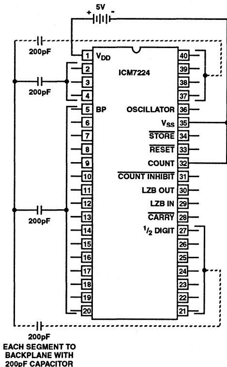
FIGURE 6. TEST CIRCUIT
