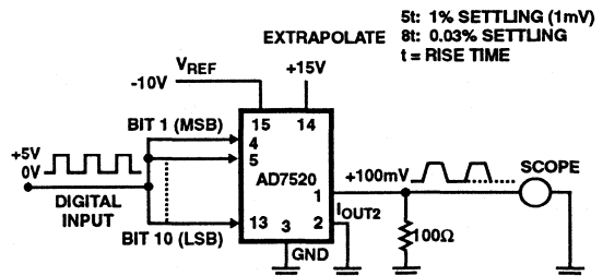
FIGURE 7. OUTPUT CURRENT SETTLING TIME
