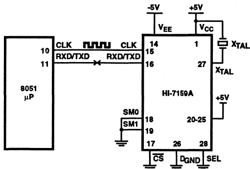
FIGURE 4A. SERIAL MODE 0
