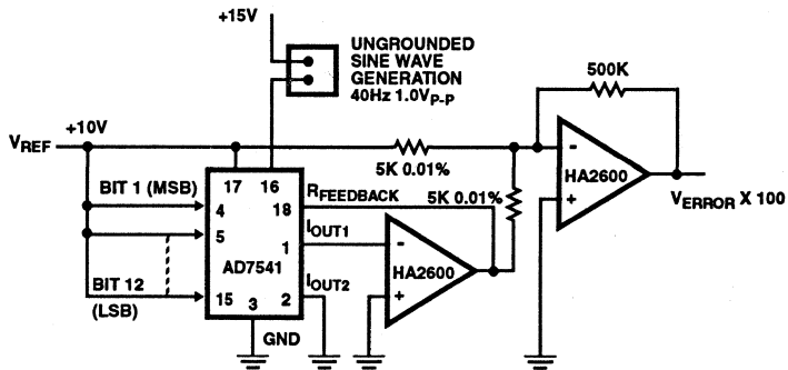
FIGURE 5. POWER SUPPLY REJECTION TEST CIRCUIT
