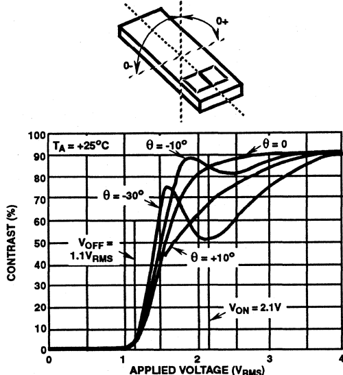
FIGURE 8. CONTRAST vs APPLIED RMS VOLTAGE
