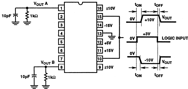
FIGURE 6. SWITCHING TIME TEST CIRCUIT
