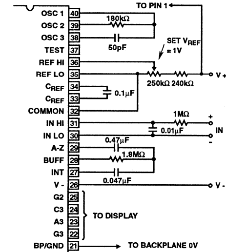
FIGURE 12. HI7131 AND HI7133 USING THE INTERNAL REFERENCE
