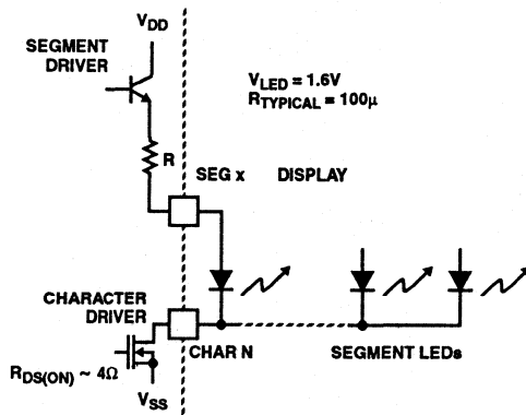
FIGURE 13. SEGMENT AND CHARACTER DRIVERS OUTPUT CIRCUIT
