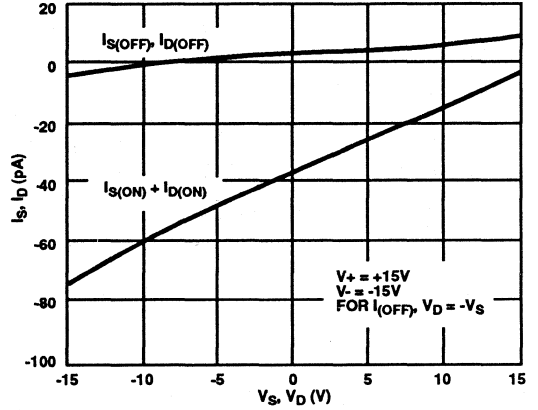
FIGURE 10. SOURCE/DRAIN LEAKAGE CURRENTS
