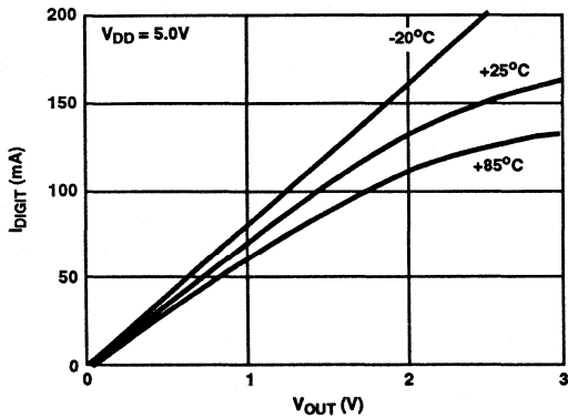
FIGURE 6. ICM7226B TYPICAL I_{DIGIT} vs V_{OUT}
