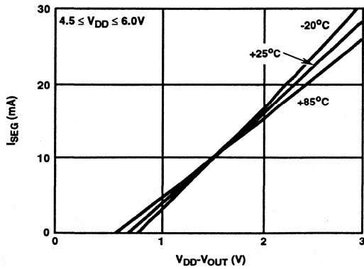
FIGURE 4. ICM7216B & ICM7216D TYPICAL I_{SEG} vs V_{DD}-V_{OUT}
