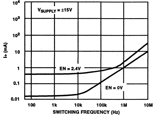
FIGURE 10. POSITIVE SUPPLY CURRENT vs SWITCHING FREQUENCY
