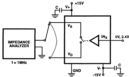
FIGURE 12. SOURCE/DRAIN CAPACITANCES
