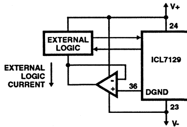
FIGURE 5. BUFFERED DGND
