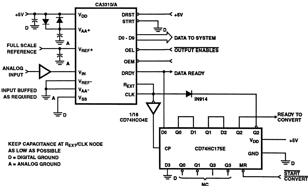
FIGURE 21. DIGITAL TRACK-AND-HOLD BLOCK DIAGRAM
