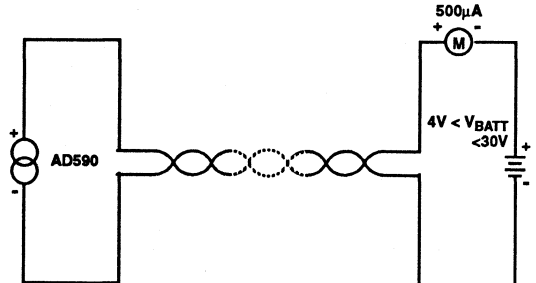
FIGURE 10. SIMPLEST THERMOMETER.
