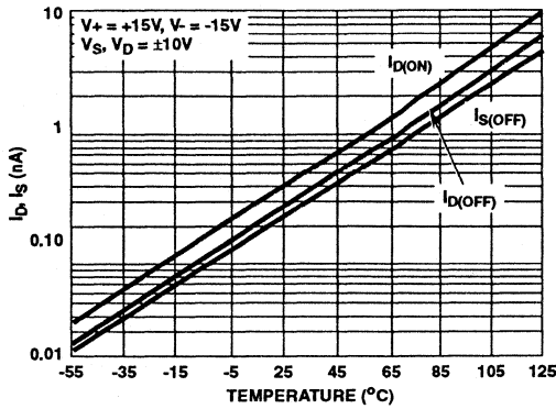
FIGURE 7. LEAKAGE CURRENT vs TEMPERATURE
