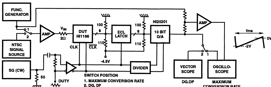
FIGURE 2. MAXIMUM CONVERSION RATE AND DIFFERENTIAL GAIN/PHASE ERROR TEST CIRCUIT
