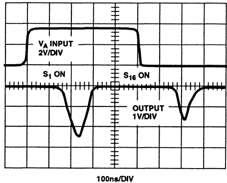
FIGURE 9C. BREAK-BEFORE-MAKE DELAY ( t_{OPEN} )
