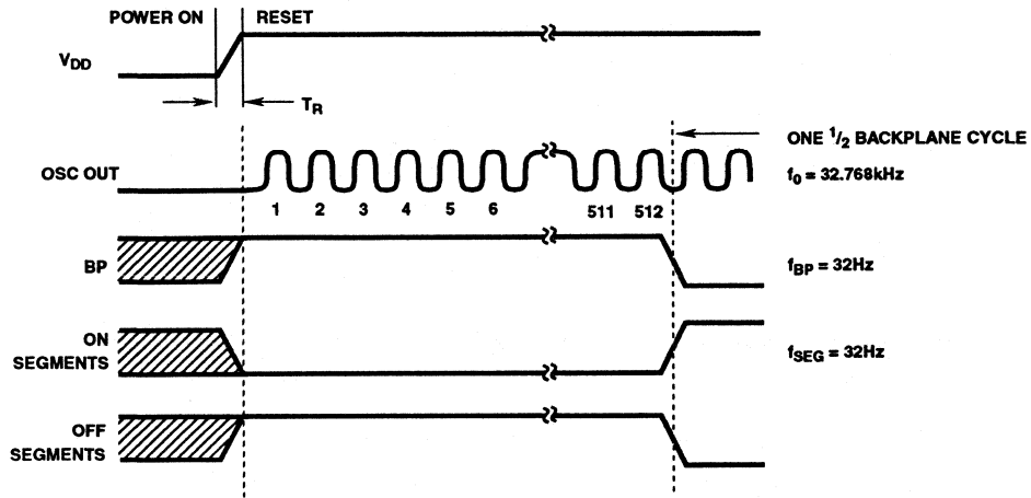
FIGURE 1. POWER ON/RESET WAVEFORMS
