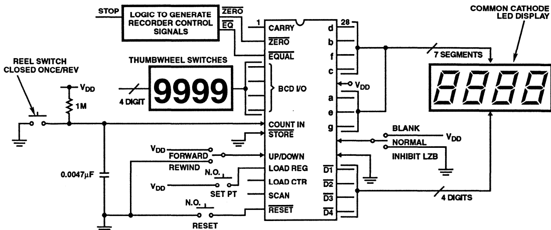
FIGURE 20. TAPE RECORDER POSITION INDICATOR
