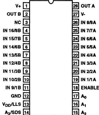
HI-516 (CDIP, PDIP, SOIC) TOP VIEW
