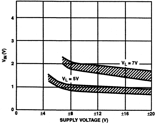
FIGURE 1. SWITCHING THRESHOLD vs SUPPLY VOLTAGE
