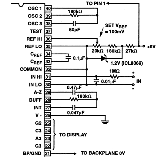
FIGURE 13. HI7131 AND HI7133 WITH AN EXTERNAL BAND-GAP REFERENCE (1.2V TYPE)
