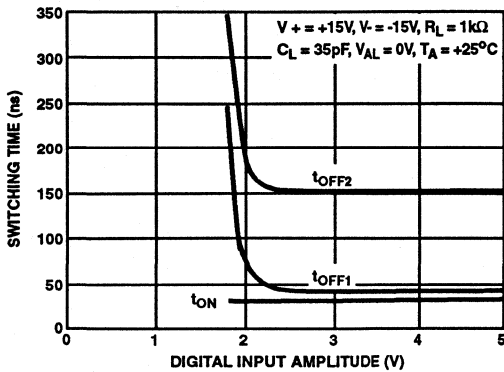
FIGURE 14. SWITCHING TIME vs INPUT LOGIC AMPLITUDE
