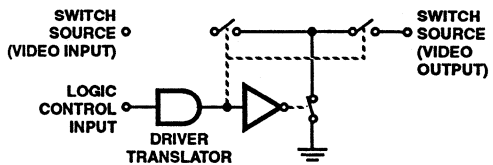
FIGURE 6. INTERNAL SWITCH CONFIGURATION
