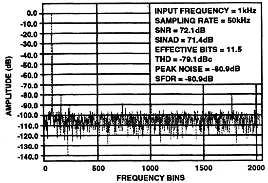
FIGURE 13. FFT SPECTRUM
