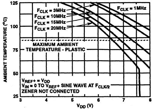
FIGURE 5. TYPICAL MAXIMUM AMBIENT TEMPERATURE AS A FUNCTION OF SUPPLY VOLTAGE
