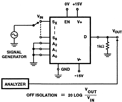
FIGURE 29. OFF ISOLATION
