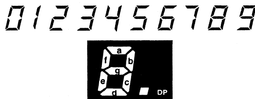
FIGURE 12. SEGMENT IDENTIFICATION AND DISPLAY FONT
