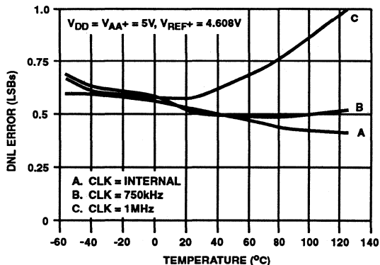
FIGURE 8. DNL vs TEMPERATURE
