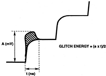
FIGURE 7. GLITCH ENERGY
