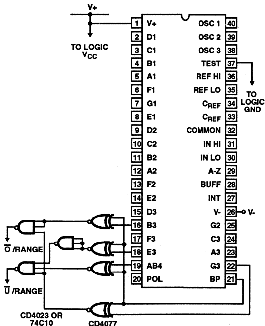
FIGURE 19. CIRCUIT FOR DEVELOPING UNDER-RANGE AND OVERRANGE SIGNAL FROM ICL7136 OUTPUTS
