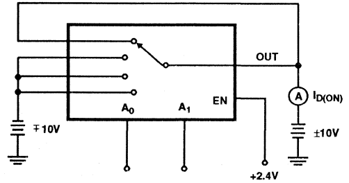
TEST CIRCUIT 4. LEAKAGE CURRENT (NOTE 1)
