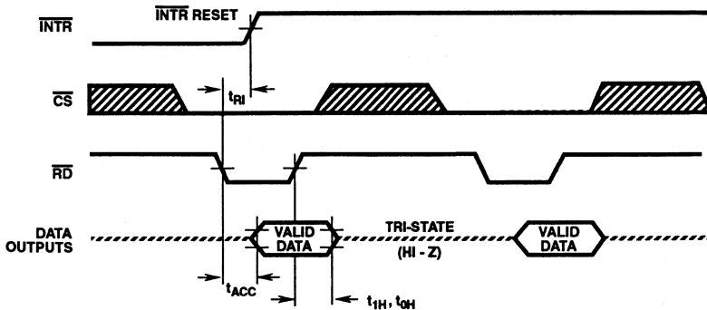
FIGURE 10B. OUTPUT ENABLE AND RESET \overline{\text{INTR}}
