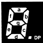
FIGURE 10. DIGITS SEGMENT ASSIGNMENTS
