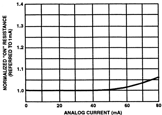
FIGURE 7. NORMALIZED "ON" RESISTANCE vs ANALOG CURRENT
