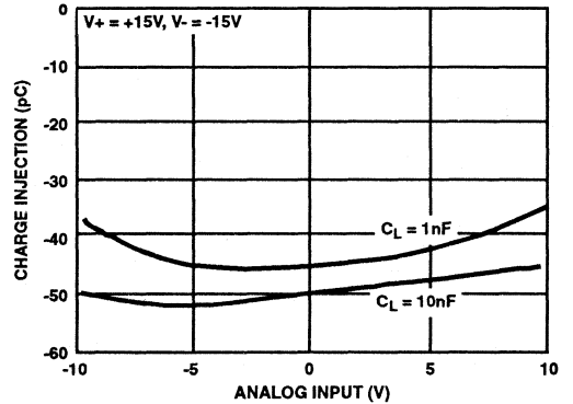
FIGURE 10. Q_{INJ} vs V_S
