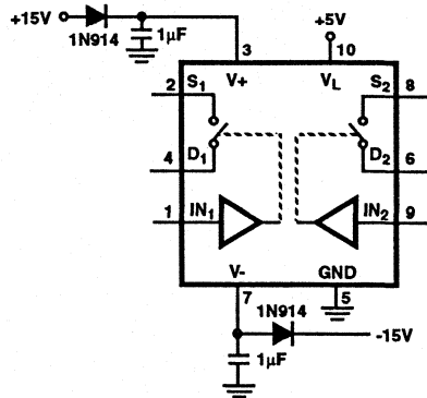
FIGURE 13. OVERVOLTAGE PROTECTION
