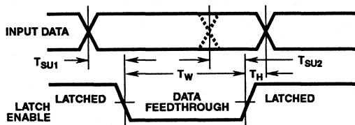
FIGURE 1. DATA TO LATCH ENABLE TIMING
