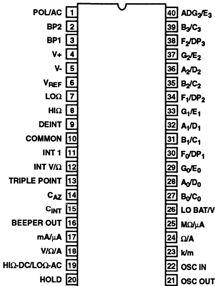
ICL7139 AND ICL7149 (PDIP) TOP VIEW
