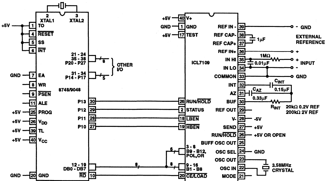
FIGURE 1B. TYPICAL CONNECTION DIAGRAM PARALLEL INTERFACE WITH 8048 MICROCOMPUTER
