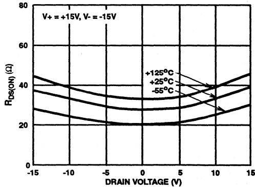
FIGURE 1. R_{DS(ON)} vs V_D AND TEMPERATURE
