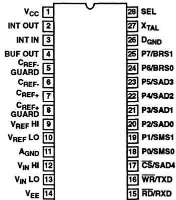
HI-7159A (PDIP) TOP VIEW
