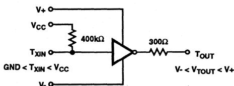
FIGURE 5. TRANSMITTER
