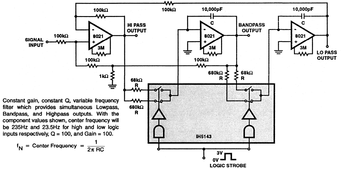
FIGURE 21. DIGITALLY TUNED LOW POWER ACTIVE FILTER
