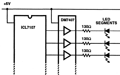
FIGURE 22. DISPLAY BUFFERING FOR INCREASED DRIVE CURRENT
