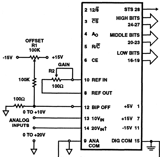
FIGURE 2. UNIPOLAR CONNECTIONS
