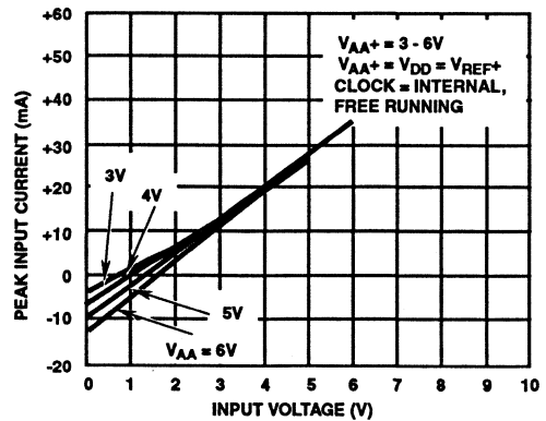
FIGURE 9. AVERAGE INPUT CURRENT vs INPUT VOLTAGE
