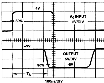
FIGURE 6. ACCESS TIME
