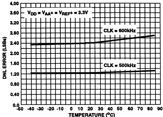
FIGURE 7. DNL vs TEMPERATURE
