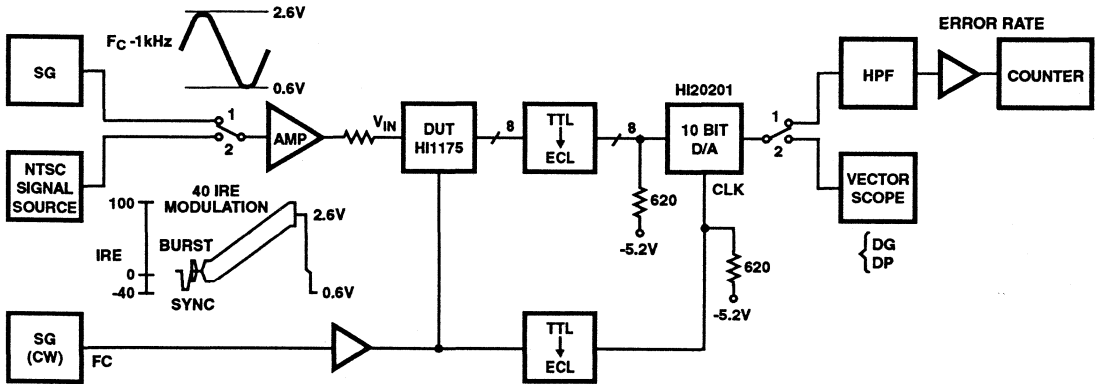
FIGURE 7. MAXIMUM OPERATIONAL SPEED AND DIFFERENTIAL GAIN AND PHASE ERROR TEST CIRCUIT
