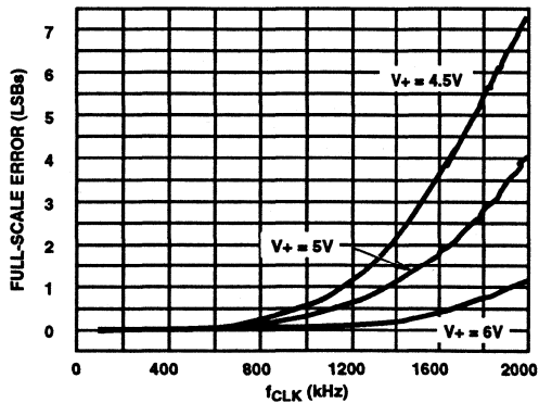
FIGURE 6. FULL SCALE ERROR vs f_{\text{CLK}}
