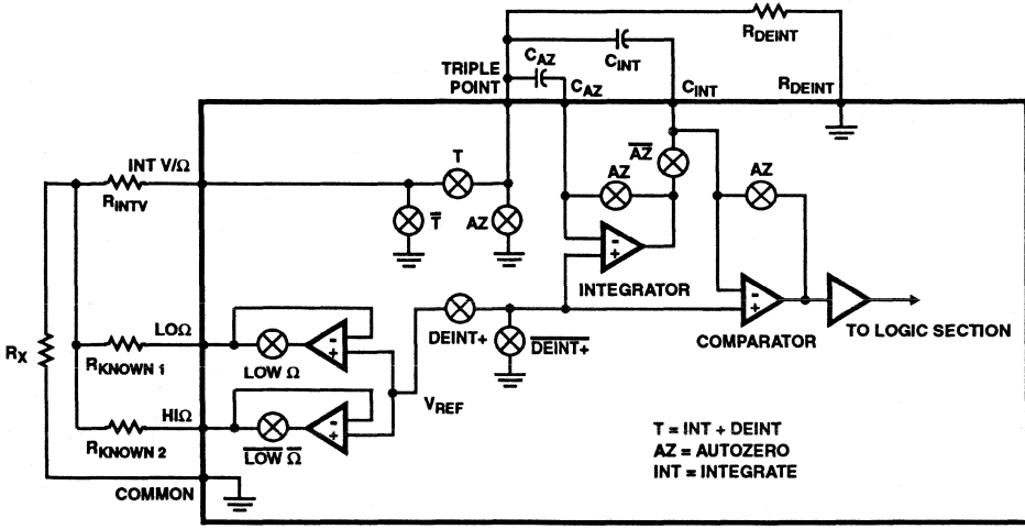
FIGURE 8. DETAILED CIRCUIT DIAGRAM FOR RATIOMETRIC Ω MEASUREMENT
